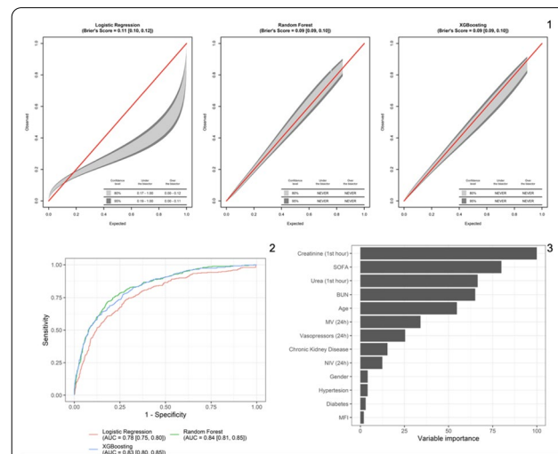
1 – Calibration belts for Logistic Regression (LR), Random Forest (RF) and eXtreme Gradient Boosting (XGB); 2 – Receiver Operating Characteristic (ROC) and Area Under the Curve (AUC) curves; 3 – Variables' importance for the Random Forest model.
