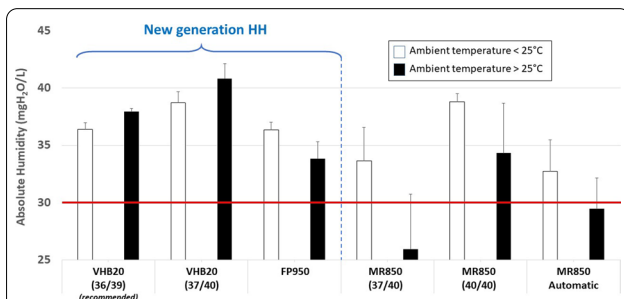
Figure: Absolute Humidity at different ambient temperatures (above and below 25 °C) delivered by new generation heated humidifiers (VHB20 and FP950) and previous generation (MR 850 at different settings: 37/40, 40/40 and with compensation activated). The minimum recommended absolute humidity (30 mgH 2 O/L) is represented by a red line.
