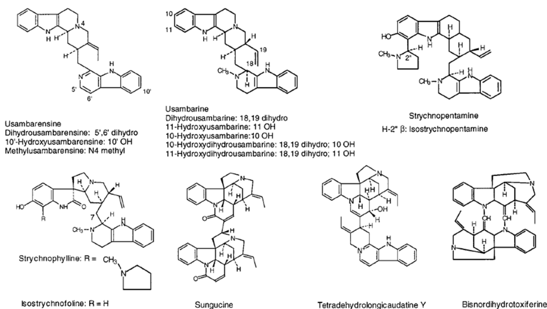
Figure 1. Chemical structures of Strychnos alkaloids.
