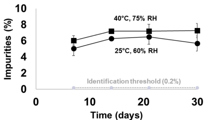
Fig. 12. Average amount of total impurities observed over four weeks at 25 °C 60 % RH (○) and 40 °C, 75 % RH (□).
