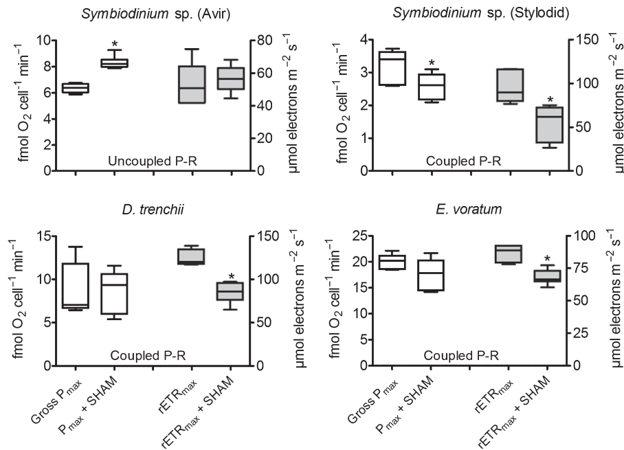
Fig. 3 Comparison of maximal gross oxygen evolution (gross P_{\text{max}} ) and maximal relative electron transport rate of photosystem II (rETR _{\text{max}} ) in Symbiodinium sp. (Avir), Symbiodinium sp. (Stylodid), Durusdinium trenchii and Effrenium voratum . Measurements were performed both in the absence and presence of salicylhydroxamic acid (SHAM), an inhibitor of mitochondrial alternative oxidase activity. All the measurements were performed for at least three independent culture replicates. Box plots show the interquartile range (box), median (horizontal line), and range (vertical bars). *, P < 0.05 .
