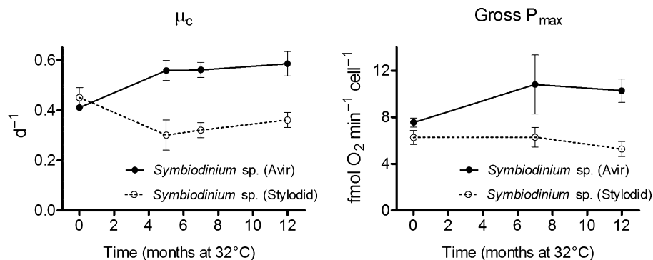
Fig. 5 Cell-specific division rate ( \mu_c ) and gross maximal photosynthesis ( P_{\max} ) of Symbiodinium sp. (Avir) and Symbiodinium sp. (Styloidid) growing at 25°C (0 months) and during the 1-yr-long experiment at 32°C. Measurements were performed for at least three independent biological replicates. The connecting line fits through the raw data. Vertical bars indicate the standard deviation.
