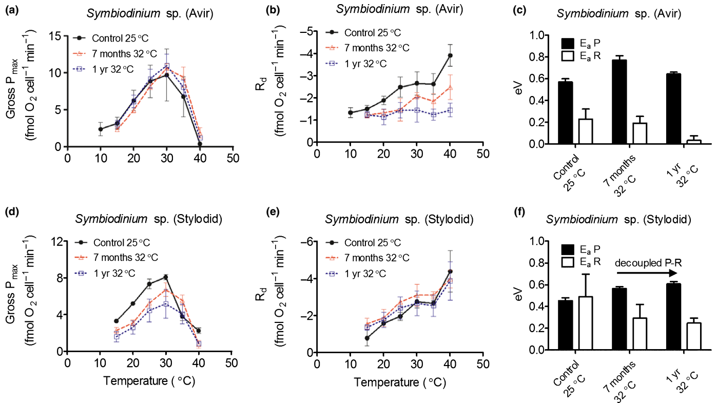
Fig. 6 Changes in thermal response curve characteristics during the 1-yr-long experiment at 32 ^{\circ}\text{C} , in comparison to cells kept at 25 ^{\circ}\text{C} . (a, d) Gross maximal photosynthesis ( P_{max} ) of Symbiodinium sp. (Avir) and Symbiodinium sp. (Stylodid). (b, e) Respiration ( R_d ) of Symbiodinium sp. (Avir) and Symbiodinium sp. (Stylodid). (c, f) Activation energies of gross photosynthesis ( E_a P ) and respiration ( E_a R ) of Symbiodinium sp. (Avir) and Symbiodinium sp. (Stylodid). All measurements were performed for at least three independent culture replicates. The connecting line fits through the raw data. Vertical bars indicate the standard deviation.
