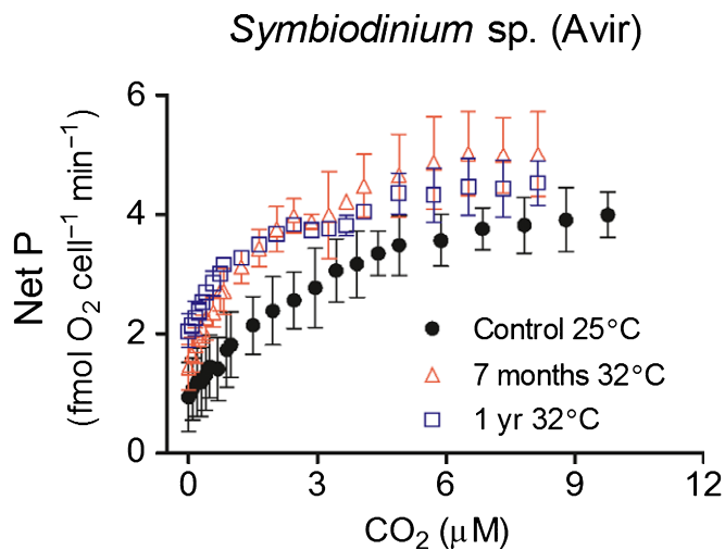
Fig. 7 Photosynthetic response to inorganic carbon ( P vs \text{CO}_2 curves) of Symbiodinium sp. (Avir) when exposed to 25 ^{\circ}\text{C} temperature conditions and during the 1-yr-long experiment at 32 ^{\circ}\text{C} . Vertical bars indicate standard deviation of at least two independent replicates.
