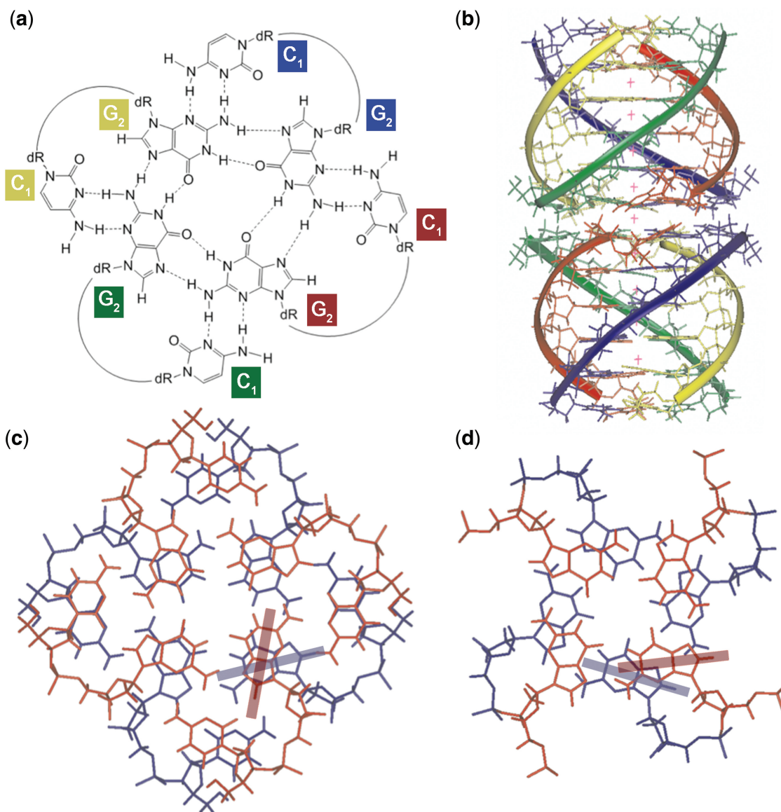
Figure 5. Structural model for the (dCGGTGGT) 8 octamer. (a) Proposed structure of the G 2 :(C 1 ):G 2 :(C 1 ):G 2 :(C 1 ):G 2 :(C 1 ) octad. (b) Molecular model of the octamer: a different color was used for each ODN strand, and potassium ions appear as red crosses. (c) Detail of stacking of the octads. (d) Detail of stacking of G 2 -G 3 tetrads. The transition moments of guanines corresponding to the absorption band at approximately 250 nm are shown as colored bars in (c) and (d).
