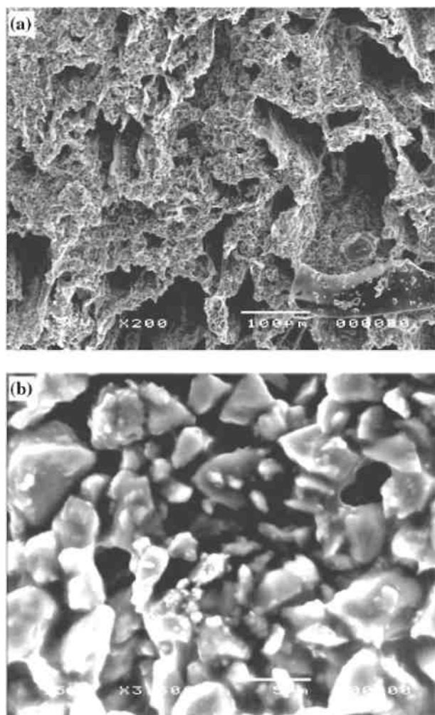
Figure 2 SEM micrographs showing the microstructure of Bioglass ® -coated PDLLA foams produced by slurry-dipping. The efficient infiltration of Bioglass ® particles into the pores (a) and the homogeneous coating microstructure (b) can be observed.
