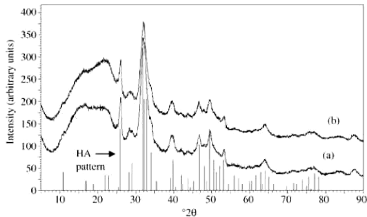
Figure 5 XRD pattern of Bioglass ® -filled PDLLA foam composites (40 wt % Bioglass ® content) after immersion in PBS for 7 (a) and 28 (b) days, showing development of HA crystals. Note that the intensity is given in arbitrary units, i.e. the relative height of the peaks does not correlate with the relative amount of HA present in the different samples.
