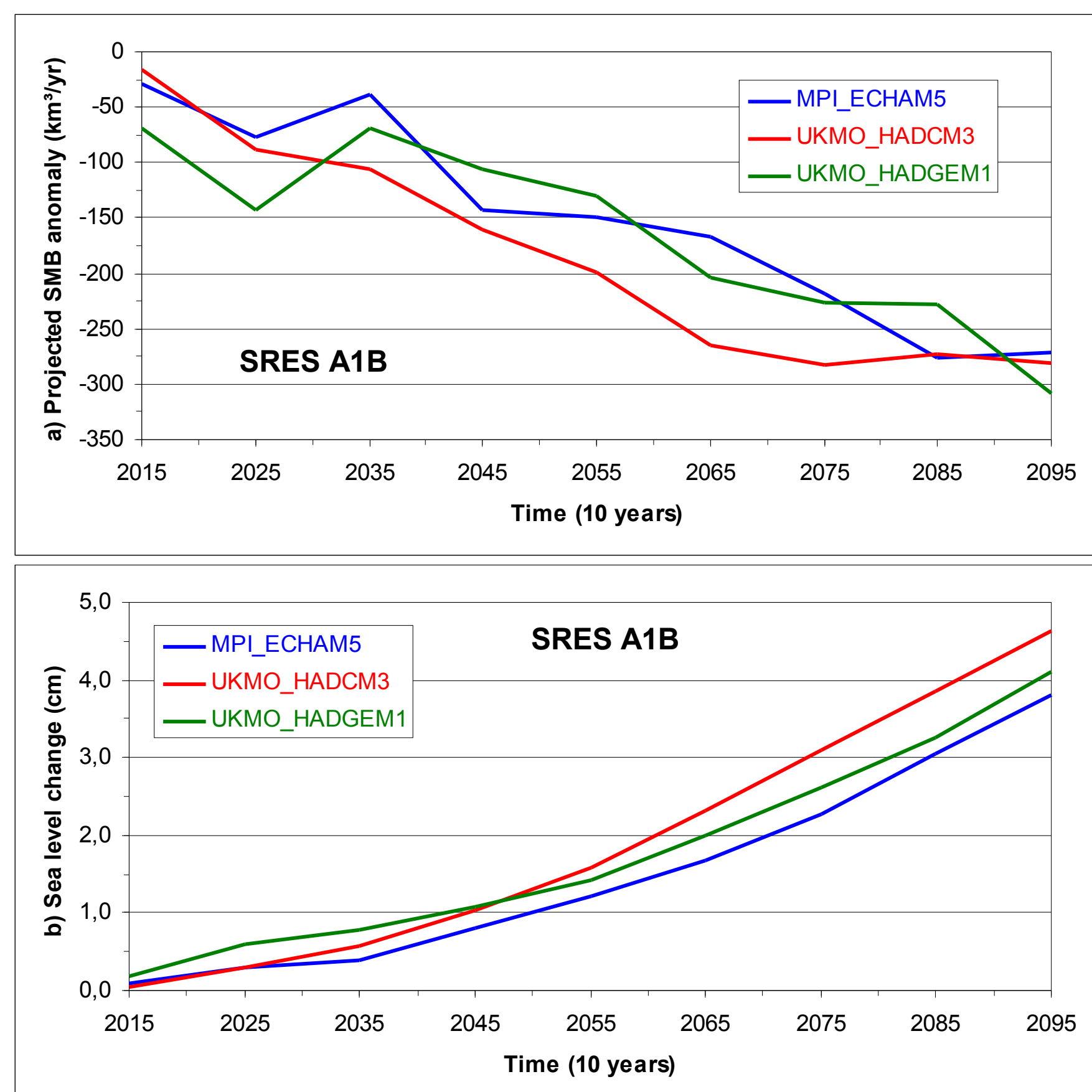
Fig. 5 : (a) Time series of SMB anomalies projected by the AOGCM's outputs. The anomalies are decadal means and refer to 1970-1999 period where the mean SMB rate is estimated to be ~ 350 km³/yr. (b) The same as a) but for the projected GrIS SMB changes expressed in equivalent sea-level rise (in cm). The computation was made by using an area of a world ocean of 361 million km².
