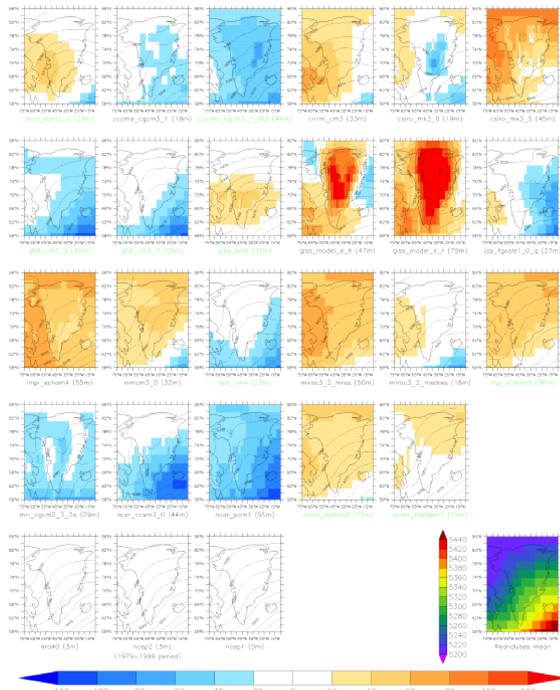
Fig. 1 : Anomalies (in m) between the annual 500hPa geopotential height simulated by the AOGCM's from the 20C3M Experiment outputs, and the annual 500hPa geopotential height from the reanalyses mean, for the 1970-1999 period. In brackets, the average of absolute anomalies compared to the reanalyses mean over the GrIS. The 500hPa geopotential height (in m) is marked in dashed lines. In green, the efficient AOGCM's to the atmospheric circulation modeling.
