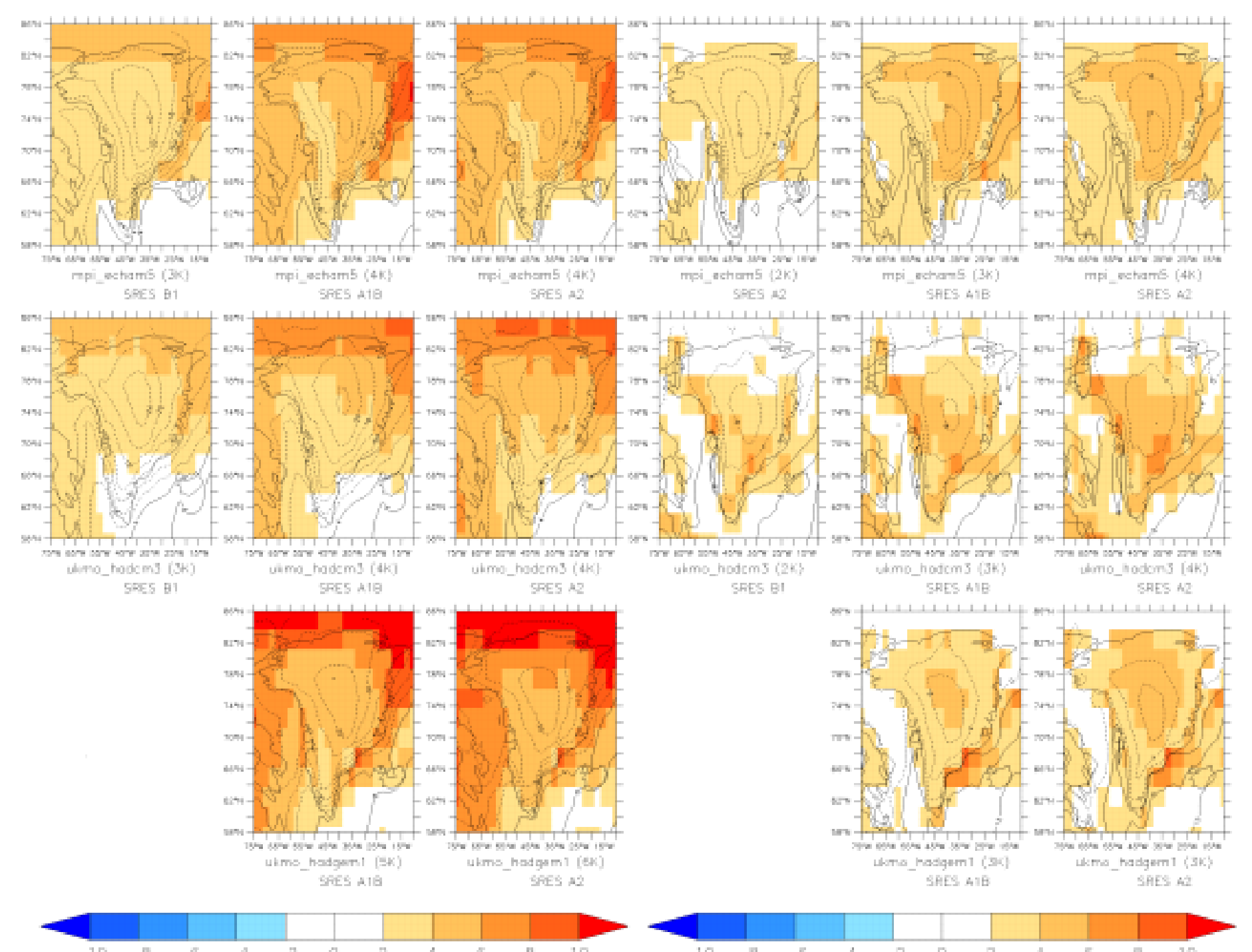
Fig. 4 : (a) AOGCM's anomalies (in °K) of the annual near surface temperature (for the 2070-2099 period) compared to AOGCM's near surface temperature for the present climate. Projected near surface temperatures (in °C) are marked in continuous lines (positive temperatures) and in dashed lines (negative temperatures). In brackets, the average of anomalies compared to the 1970-1999 period over the GrIS. (b) The same as a), but for the projected precipitation expressed in mm. In brackets, the amount of precipitation anomalies over the GrIS.
