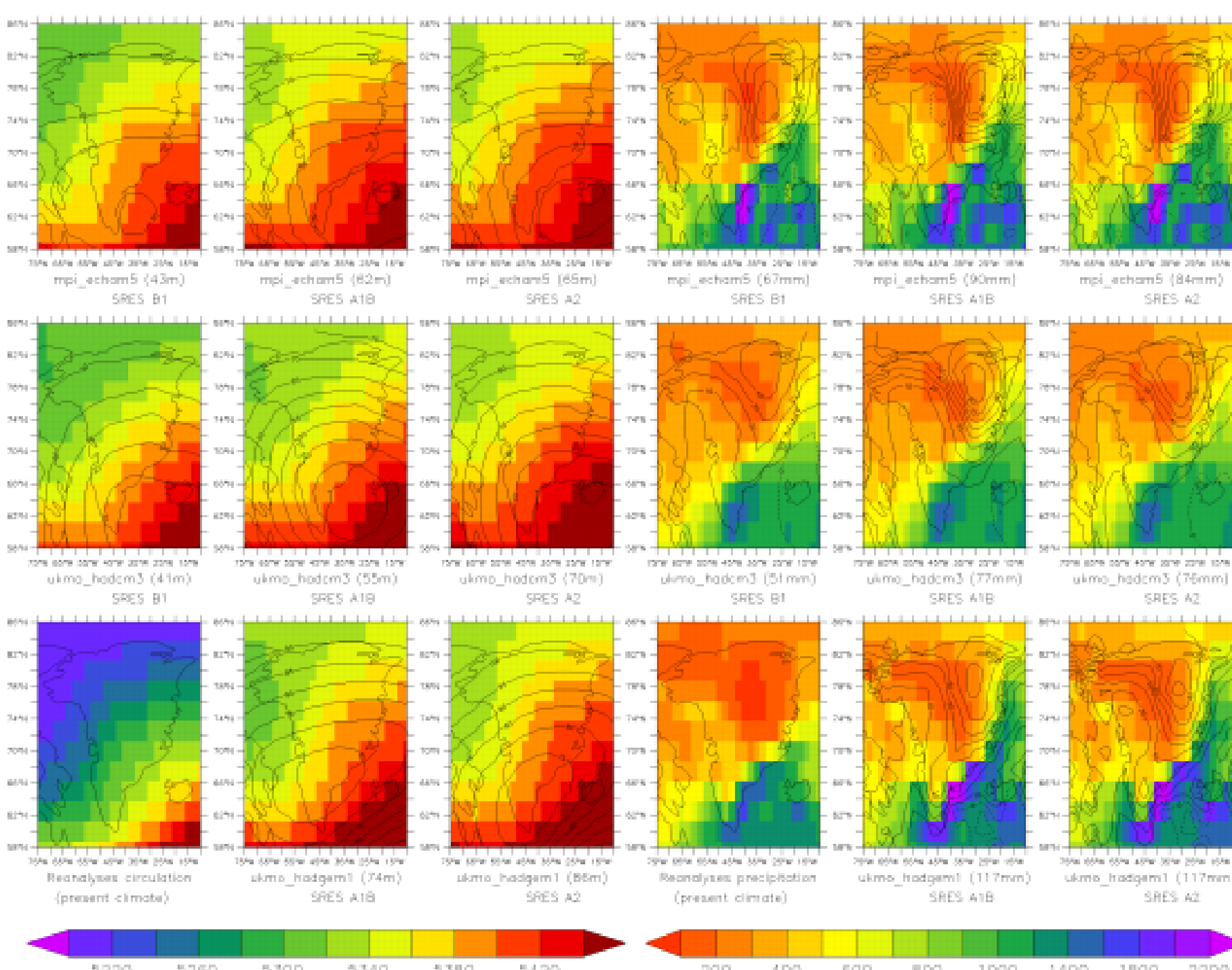
Fig. 3 : (a) Annual 500hPa geopotential height (in m) simulated by the selected AOGCM's from SRES scenarios for the 2070-2099 period. Anomalies (in m) compared to the AOGCM's 500hPa geopotential height for the present climate are marked in continuous lines (positive anomalies) and in dashed lines (negative anomalies). In brackets, the average of anomalies compared to the 1970-1999 period over the GrIS. (b) The same as a), but for the projected precipitation expressed in mm. In brackets, the amount of precipitation anomalies over the GrIS.
