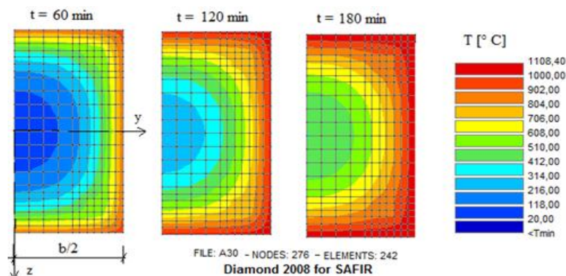
Figure 6. Calcul iso thermal aux temps : t = 60, 120, 180min
