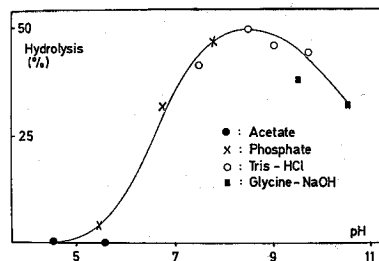
FIGURE 5: pH optimum of DD-carboxypeptidase from Streptomyces R39. All the buffers were used at 0.02 M. N^\alpha, N^\epsilon -Diacetyl-L-lysyl-D-alanyl-D-alanine (40 nmoles) was incubated at 37° for 1 hr in the presence of 0.65 \mu l of the enzyme solution after step 2, in a final volume of 35 \mu l. Results are expressed in per cent of hydrolysis.
