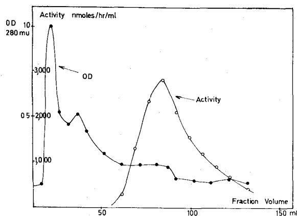
FIGURE 3: Purification of DD-carboxypeptidase from Streptomyces K11. Elution from polyacrylamide gel after electrophoresis (height of the gel: 4 cm; for conditions, see text) (step 4). For enzyme estimation, see Figure 1 except that 10 \mu l of effluent fractions were incubated with the peptide for 90 min.
