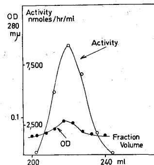
FIGURE 2: Purification of DD-carboxypeptidase from Streptomyces R39. Filtration on a 400-ml Sephadex G-75 column (step 4). For enzyme estimation, see Figure 1 except that 9 \mu l of effluent fractions were incubated with the peptide for 25 min.
