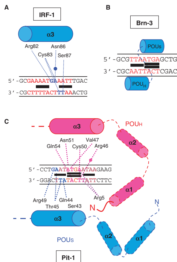
Figure 8. Diagrams for hypothesized positioning of the protein and identified binding of DB293 on the various consensus-binding sites. The position of DB293 over IRF-1 (A), Brn-3 (B) and Pit-1 (C) consensus-binding sites (in red) are presented as black boxes stacking as monomers or dimers in the minor groove of the DNA. The points of interaction between the amino acids implicated in the DNA recognition and the specific target sequences are presented as dashed lines. The water molecules implicated in the interaction are presented as full circles. In blue or pink are the DNA bases implicated in the protein direct interaction. Blue and pink dashed lines correspond to interaction bonds within the major groove of the DNA whereas purple dashed lines correspond to interaction bonds within the minor groove.
