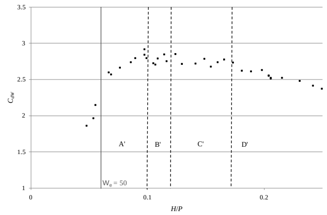
Figure 10 Discharge coefficient C_d for low heads with A' leaping nappe, B' springing nappe on lateral crest, C' springing nappe on lateral and downstream crests, D' springing nappe all over the crest Same as Fig. 9
