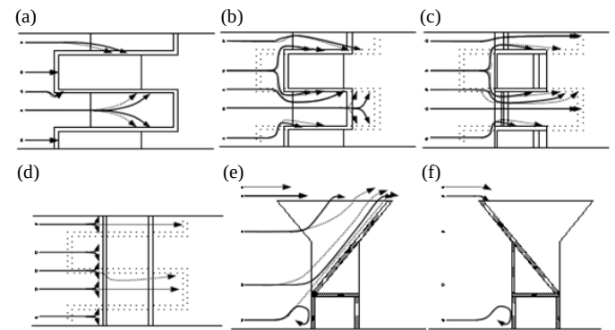
Figure 5 Streamlines for (—→) low ( H/P \leq 0.2 ) and (---→) high heads ( H/P > 0.2 ) at different weir height (a) z = 72.5 cm, (b) z = 55 cm, (c) z = 25 cm, (d) z = 5 cm and along the inlet (e) and the outlet (f).
