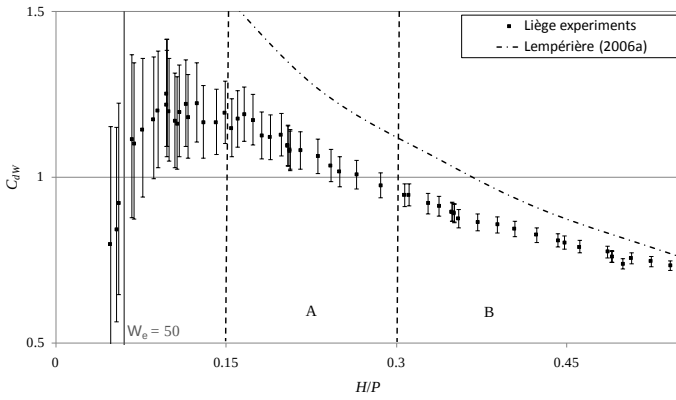
Figure 4 Non-dimensional head/discharge relation regarding Liège experiments ( L/W = 4.15 , W_i/W_o = 1 , W_u/P = 0.76 , B_o/B_i = 1 ) and Lempérière (2006a) results ( L/W = 4 , W_i/W_o = 1 , W_u/P = 1.1 , B_o/B_i = 1 ) with decrease region A and stabilization region B.
