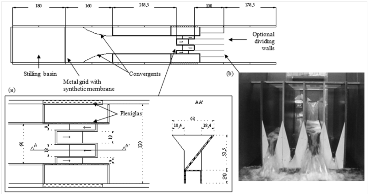
Figure 2 Test set-up (a) plan of PKW model, (b) optional sharp-crested triangular weirs (Lengths in cm) Lettering looks poor, drop colour+épaisseurs
