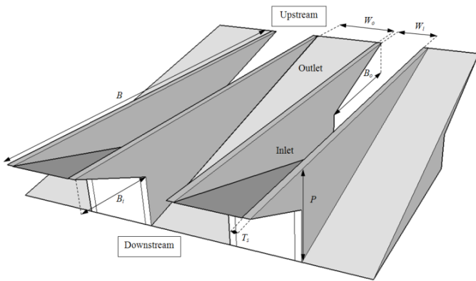
Figure 1 3D sketch of PKW with main geometric parameters
