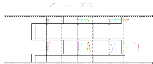
Figure 11 Froude number profiles over PKW (red - H/P = 0.5 ; green - H/P = 0.35 ; blue - H/P = 0.2 ; pink - H/P = 0.1 ; broken lines - Fr^2 = 1 ) Same
