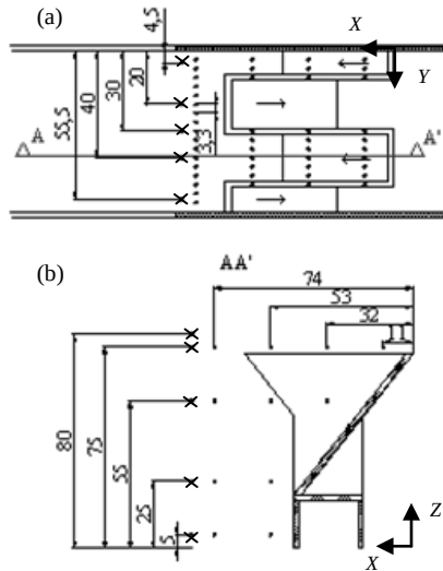
Figure 3 (x) Dye supply and (•) Pitot measurement locations (a) plan, (b) inlet section (Distances in cm) Same
