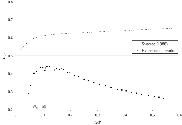
Figure 9 Comparison between crest efficiencies of tested model and linear weir, (l) limit of surface tension effects W_e = 50 Improve plot in black, Stop at 0.7 ADD vertical line on right side Increase lettering size
