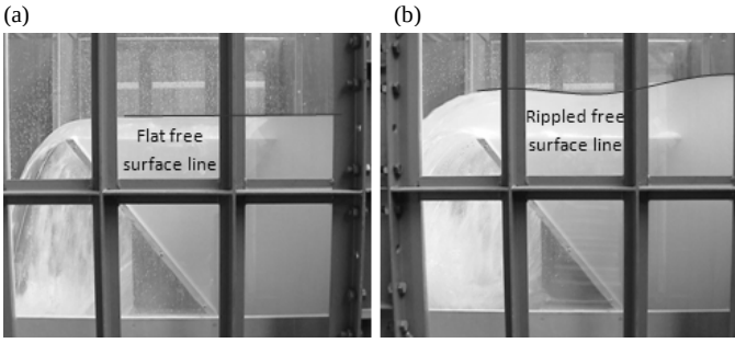
Figure 6 Free surface profiles for low and high heads of H/P = (a) 0.15, (b) 0.35 ADD (a) etc. into plots. Also, drop text from these
