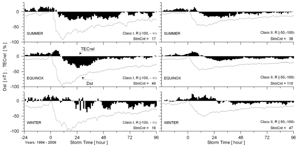
Fig.2. GPS TEC relative deviations ( TEC_{rel} ) from 27-day medians during geomagnetic storms of class I (left panels) and class II (right panels) in summer (top), equinox (middle), and winter (bottom) for the site of the IGS station DOUR (4.6°E, 50.1°N) based on data from the 1994-2009 period.
