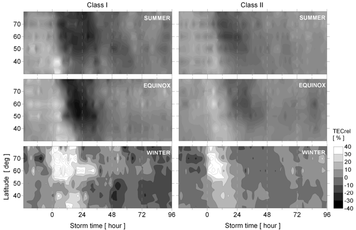
Fig.4. Latitude ( 0^{\circ}\text{E} , 30^{\circ}\text{-}80^{\circ}\text{N} ) vs storm time dependence of the GPS TEC relative deviation ( \text{TEC}_{\text{rel}} ) from 27-day medians during class I (left panels) and class II (right panels) storms in summer (top), equinox (middle), and winter (bottom) based on IGS data from the 1998-2009 period.
