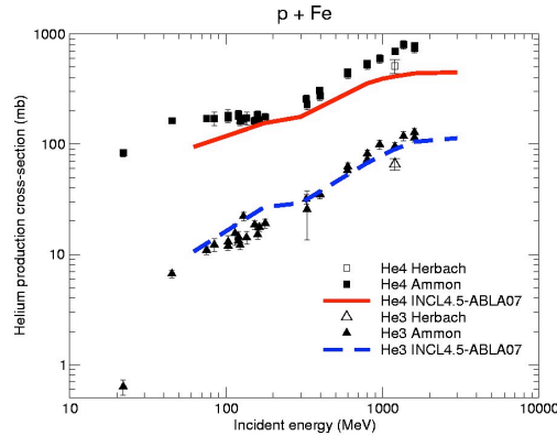
Figure 4: Helium excitation functions: Fe(p,x \alpha ). INCL4.5/Abla07 is plotted as solid line for ^4\text{He} and as dashed line for ^3\text{He} . References on Data in [13].
