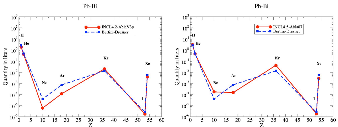
Figure 8: Quantity of volatiles (up to Xe) produced in the LBE target after 123 days of irradiation with 575 MeV protons at 0.947 mA using on the left part INCL4.2-AblaV3p and on the right part INCL4.5-Abla07. Bertini-Dresner, as default option in MCNPX, is also plotted.
