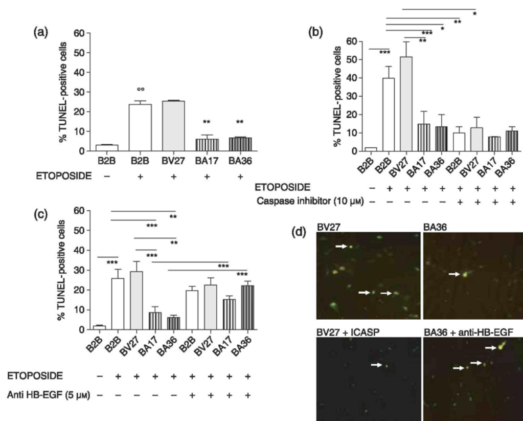
Figure 4. Representative results of TUNEL assay, measuring role of ADAM-12, in cell resistance to etoposide-induced apoptosis, effects of general caspase inhibition and HB-EGF neutralization, (a) Cells were immunostained with FITC-12-dUTP to investigate baseline or etoposide-induced apoptosis (presented data are representative of two independent experiments). Results are expressed as percentage of mean number of TUNEL-positive cells compared to total cell number for each group \pm SEM. ^{**}P < 0.01 , compared to parental or control transfected cells; ^{\circ}P < 0.01 , compared to baseline apoptosis in parental BEAS-2B cells, Mann-Whitney test, (b) Cells cultured in presence of a general caspase inhibitor and subjected to apoptosis inducing conditions showed reduced apoptotic levels when compared to standard apoptosis inducing experiments ( ^{*}P < 0.05 , ^{***}P < 0.001 ). (c) Inhibition of HB-EGF by a neutralizing antibody enhanced apoptotic levels of ADAM-12 overexpressing cells. Apoptotic levels in parental and control cells were not different when cells were cultured with etoposide alone or with etoposide and anti-HB-EGF neutralizing antibody, (d) Representative microphotographs of TUNEL staining in ADAM-12 overexpressing clones and controls. White arrows indicate examples of cells positive for TUNEL staining.
