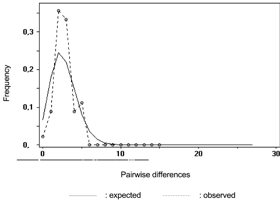
Fig. 4. Mismatch distribution for mtDNA types from the eastern genetic lineage of Mustela lutreola and the M. putorius group. The expected frequency is based on a population growth-decline model (for the groups, respectively: \theta initial = 0, 2.4, 0 and 0, \theta final = 1000, \tau = 4.4, 9.4, 2.7 and 1.6), determined using the DNASP v3.5 program (Rozas and Rozas, 1997).
