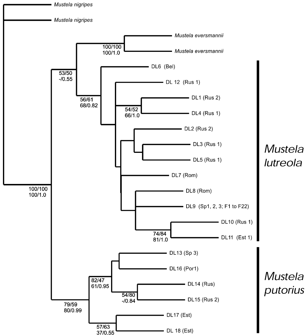
Fig. 2. Consensus tree derived from the analysis of the complete mitochondrial control region sequences for 37 European minks, polecats and black footed ferrets (used as outgroup). Each haplotype is identified by the letters DL + a specific number. The locality codes (see table 1) are also given for each haplotype. For each node supported by a least 50% of bootstrap value, the different robustness are indicated as followed:
