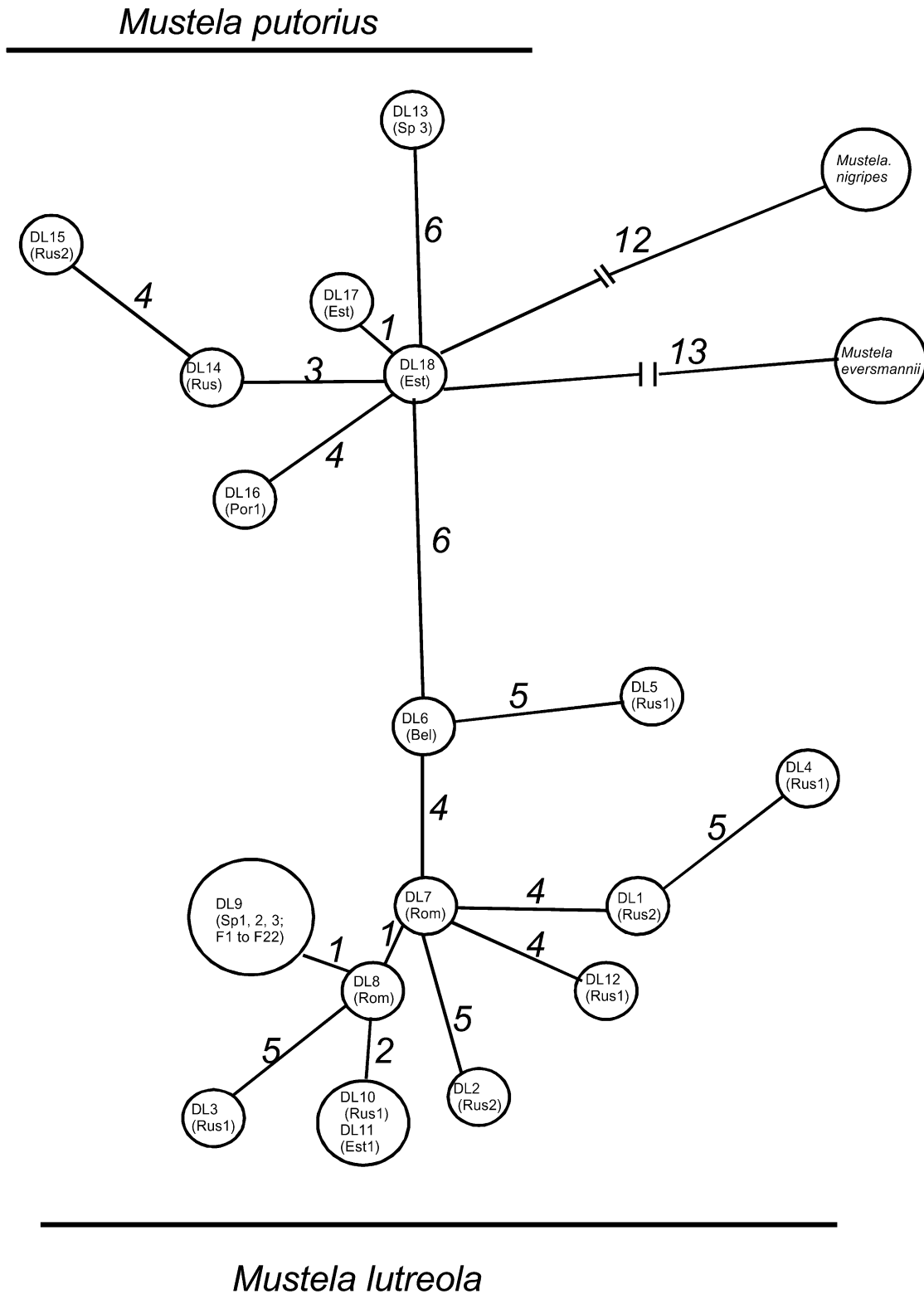
Fig. 3. A minimum spanning network constructed using mitochondrial control region sequences. The identity of the haplotypes (see Fig.s 1 and 2) and their geographic origin (see Table 1) are indicated. Numbers in italics correspond to the mutational steps observed between haplotypes.
