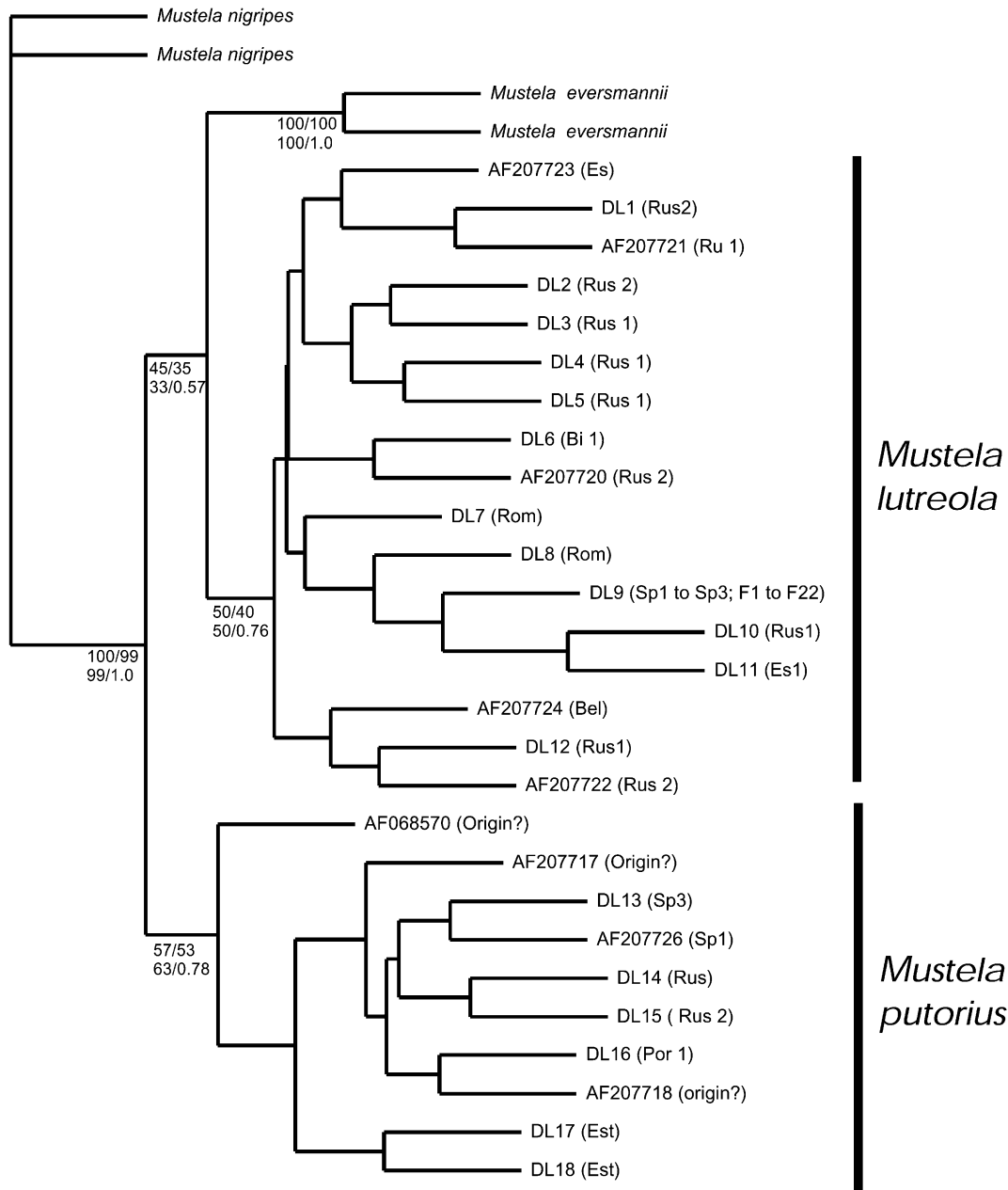
Fig. 1. Consensus tree derived from the analysis of a partial sequence of the mitochondrial control region for 57 European minks, polecats and black footed ferrets (used as outgroup). Each haplotype is identified by its accession number in GenBank or by the letters DL + a specific number. The locality codes (see Table 1) are also given for each haplotype. For each node supported by a least 50% of bootstrap value, the different robustness are indicated as followed: \frac{\text{Neighbour joining/maximum likelihood}}{\text{Maximum parsimony/Bayesian probability}} .
