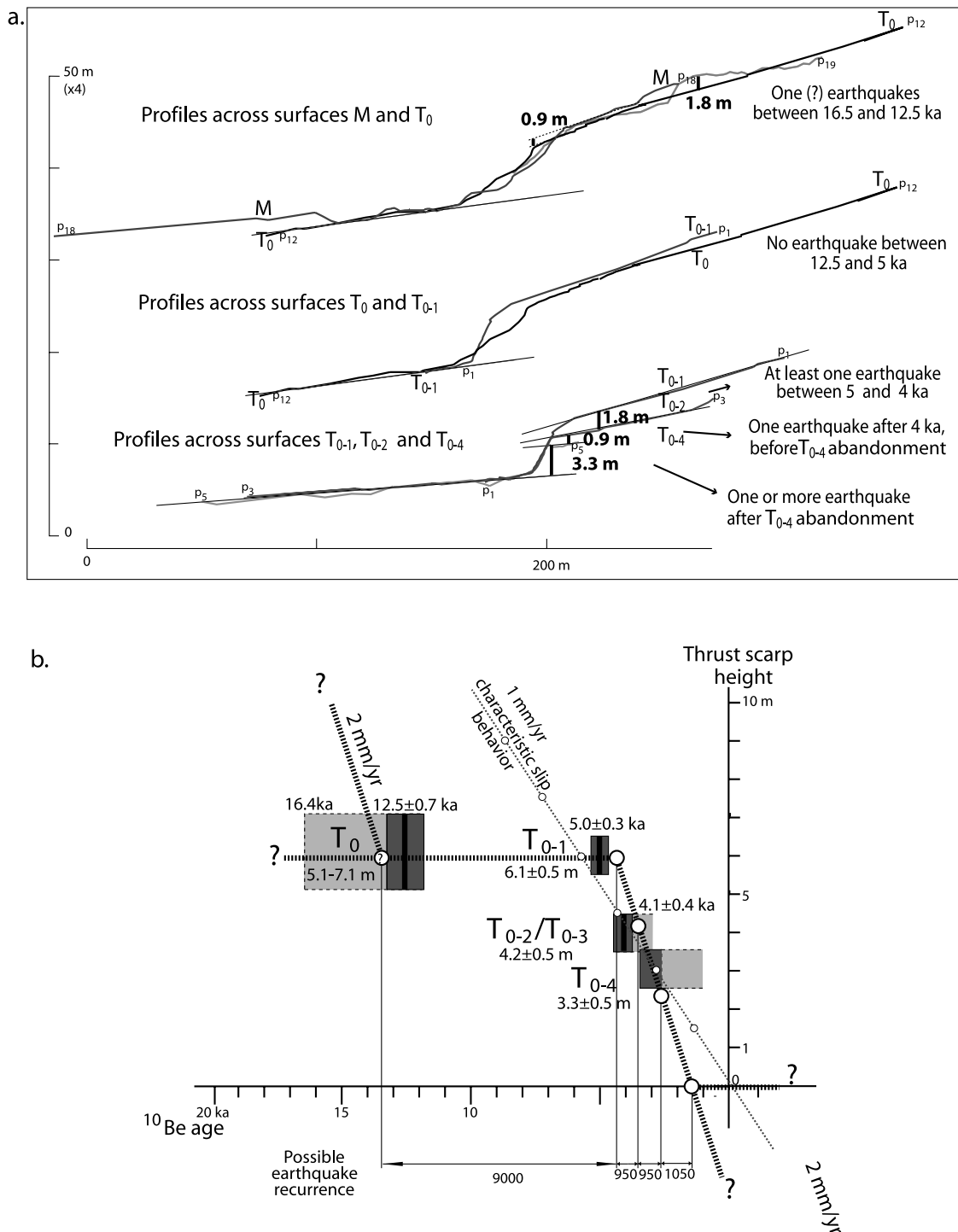
Figure 10. Seismic history for the Aksu thrust fault deduced from surface offset height and age. (a) Summary comparison of scarp height for the different surfaces and deduced seismic history, based on the profiles of Figure 6 and the surface ages of Figure 8. (b) Possible earthquake scenario (thick dashed line) with a burst of earthquakes (big white circles) during short periods of 4 to 5 ka and quiescence of at least 7500 years. Present earthquake scenario agrees with scarp heights, but many others are possible. Also shown is a scenario with a characteristic slip behavior (thin dashed line with small white circles representing characteristic earthquakes), using an average coseismic slip of about 1.5 m and a recurrence time of about 1350 years, which is not in agreement with our surface dating.
