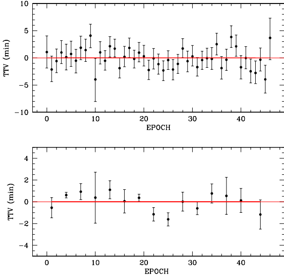
Fig. 6. Top: median value and 1- \sigma limits of the TTV posterior distributions obtained in MCMC_3 . Bottom: same curve obtained after binning the TTVs per three (error of each bin = error on the mean).
