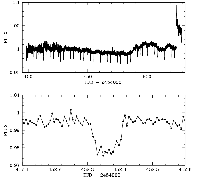
Fig. 1. Top: Normalized CoRoT LC of the star CoRoT-12. The oversampled part of the LC was binned to the same time bin than its first part for the sake of clarity. Bottom: zoom on a transit of CoRoT-12b.
