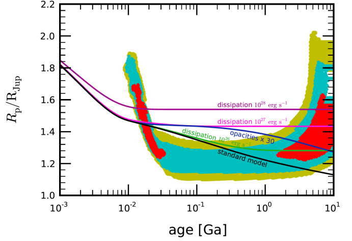
Fig. 8. Evolution of the size of CoRoT-12b (in Jupiter units, R_{Jup} ) as a function of age (in billion years), compared to constraints inferred from CoRoT photometry, spectroscopy, radial velocimetry and CESAM stellar evolution models. Red, blue and yellow-green dots correspond to the planetary radii and ages that result from stellar evolution models matching the inferred \rho_* - T_{eff} uncertainty ellipse within 1 \sigma , 2 \sigma and 3 \sigma , respectively. Planetary evolution models for a planet with a solar-composition envelope and no core are shown as plain lines and are labeled as follow : standard (black): irradiated planet with no extra heat source ; opacities x 30 (blue): opacities have been artificially multiplied by 30 compared to standard model ; dissipation : models in which 10^{26} (green), 10^{27} (pink), and 10^{28} (purple) \text{erg s}^{-1} is deposited at the planet's center. These models assume a total mass of 0.92 M_{Jup} and an equilibrium temperature of 1450 K
