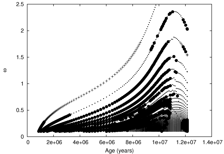
Figure 2: Dimensionless angular frequencies of degree l = 1 along the pre-main sequence. Small dots represent stable modes, filled circles correspond to excited modes without the \varepsilon -mechanism and plus signs correspond to additional excited modes when the \varepsilon -mechanism is taken into account.
