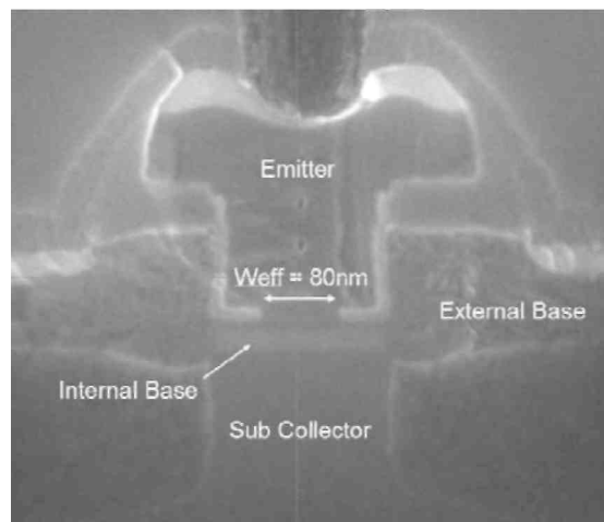
Fig. 4b. Zoom in of bipolar device after end of processing. Effective emitter window width = 80nm.
