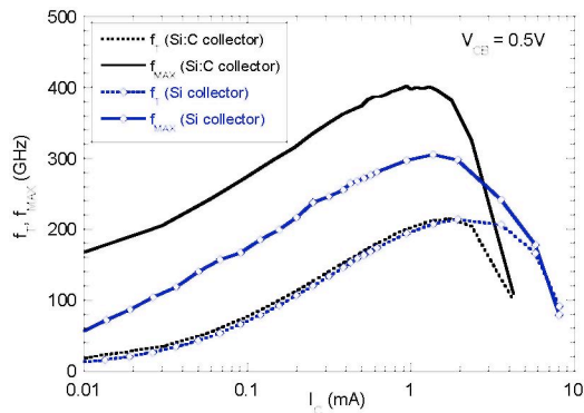
Fig. 11. f_T and f_{MAX} versus I_C for a 0.15 \times 1.0 \mu\text{m}^2 HBT.
