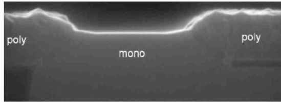
Fig. 1. Bipolar device after the single-step epitaxial growth of the collector drift and the base layer.
