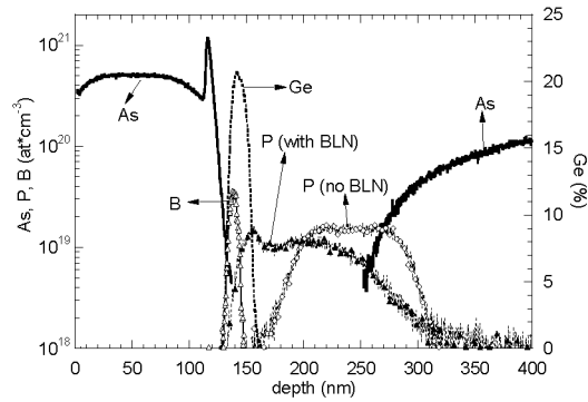
Fig. 5. EOF SIMS profiles for transistor with a Si undoped collector region underneath the base.
