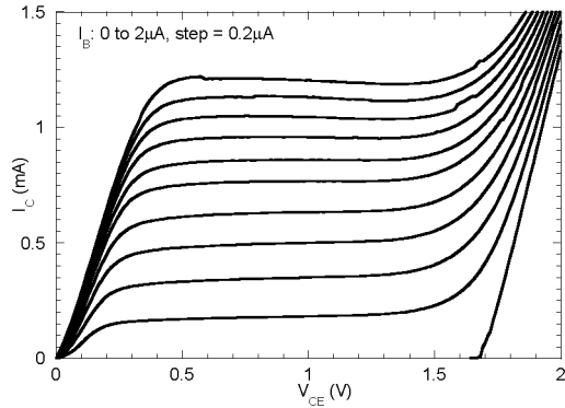
Fig. 10. I_C - V_{CE} plot with forced I_B for a 0.15 \times 1.0 \mu\text{m}^2 HBT device (Si:C collector).
