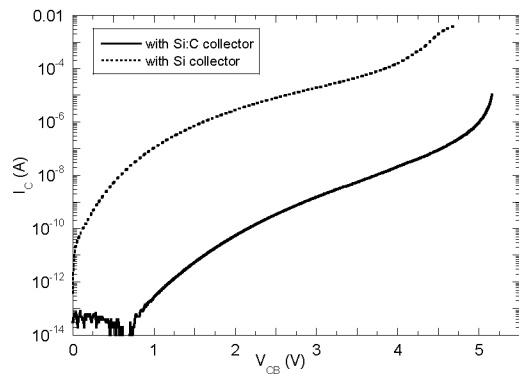
Fig. 8. Base-collector reverse diode current for a 0.15 \times 1.0 \mu\text{m}^2 HBT device.
