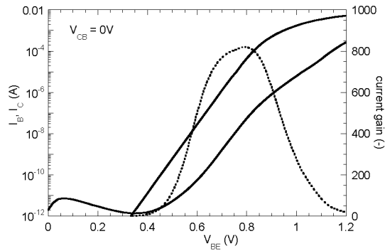
Fig. 7. Gummel plot for a 0.15 \times 1.0 \mu\text{m}^2 HBT device with Si:C collector.
