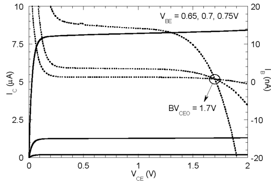
Fig. 9. I_C - V_{CE} plot with forced V_{BE} for a 0.15 \times 1.0 \mu\text{m}^2 HBT device (Si:C collector).
