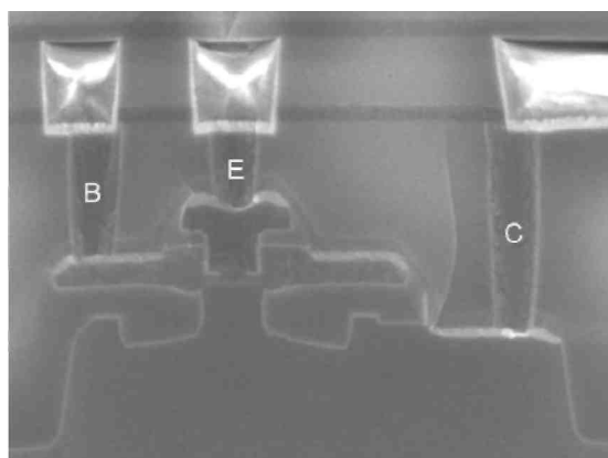
Fig. 4a. Bipolar device after end of processing in B-E-C configuration.
