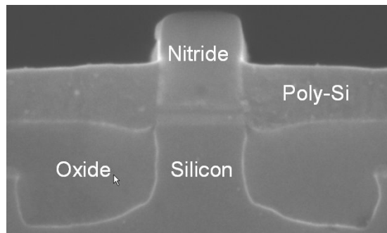
Fig. 3. Bipolar device after the poly dry etch back.
