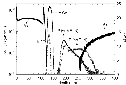
Fig. 6. EOF SIMS profiles for transistor with a Si:C undoped collector region underneath the base.
