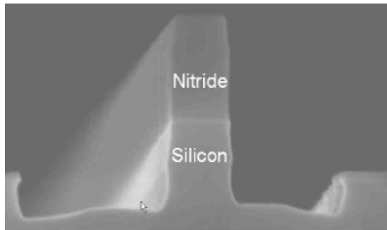
Fig. 2. Bipolar device after the pedestal etch of nitride and silicon. Width of the nitride = 150nm.
