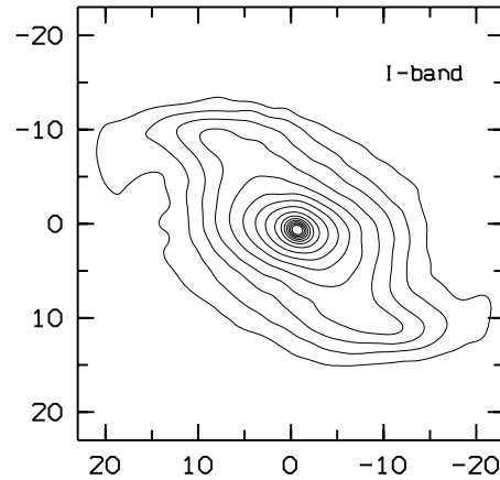
Fig. 4. Contour plots of the numerical galaxy model from the MCS deconvolution code in the I band. Both axis are in arcseconds. North is up and East is to the left.
