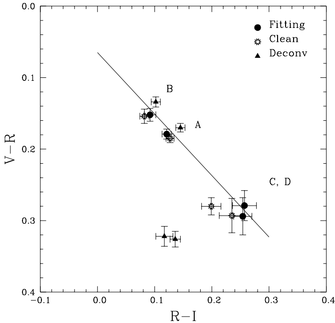
Fig. 5. V-R as function of R-I for the three different methods with errorbars on the mean of all the frames ( \sigma_{mean} in Tables 2-5). The mean extinction law for our Galaxy is drawn as a solid line through the mean colour of the A component. See Sect. 5 for an explanation of the C and D points.
