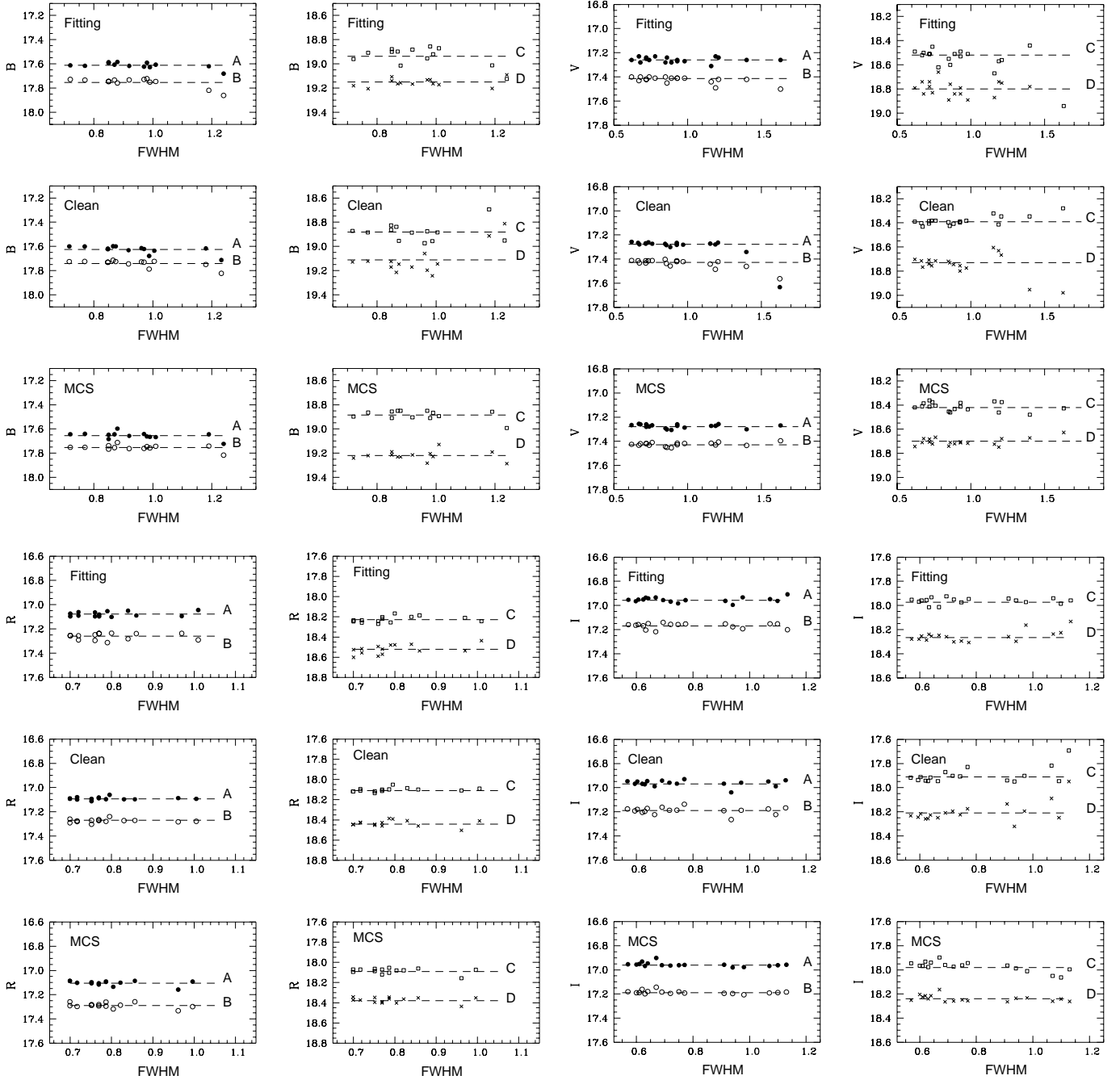
Fig. 2. Photometric magnitudes as a function of seeing (in arcseconds) for the B , V , R and I frames. Note that in the V -band, the magnitude of component D, derived with the Fitting method on the image with a seeing of 1''.63 is outside the plot.
