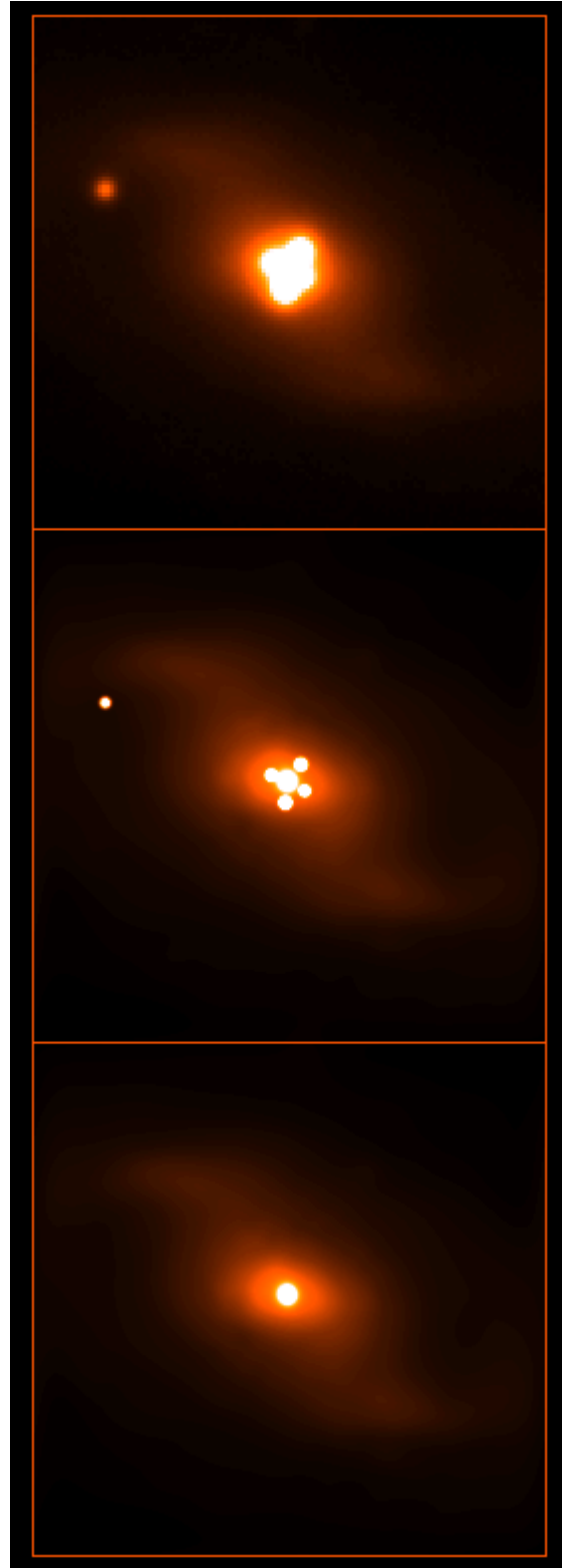
Fig. 1. [Top]: Stack of 12 R band frames with a seeing of \sim 0''.8 . [Middle]: Deconvolved frame using the MCS algorithm. The resolution is now 0''.26 . [Bottom]: Deconvolved numerical galaxy model. All the images are \sim 22'' on a side, North is up and East is to the left.
