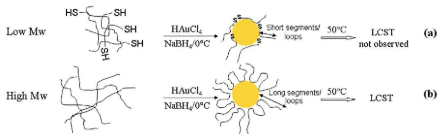
Scheme 2. Train-loop-tail model for the adsorption of PNIPAM onto the gold surface.
