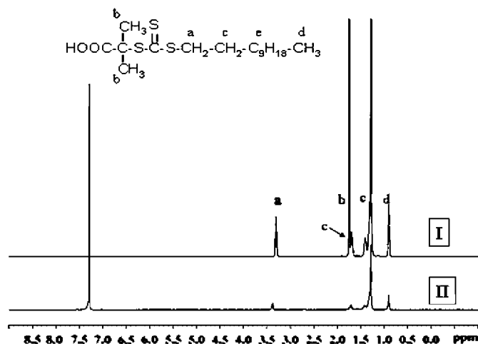
Fig. 2. ^1\text{H} NMR spectrum of DMP (a RAFT agent), before (I) and after (II) hydrolysis in water at pH ~ 10.
