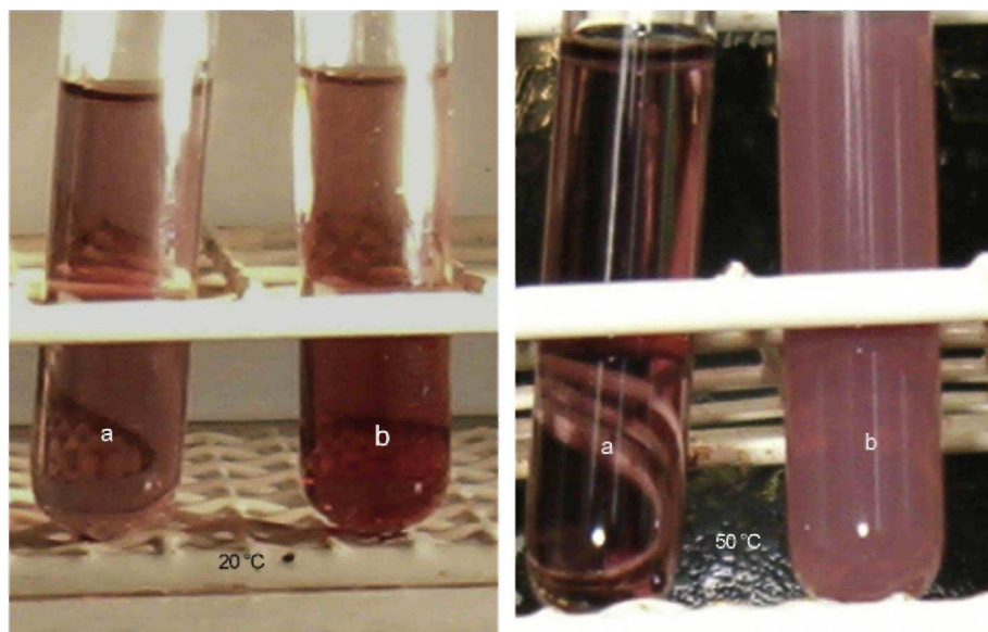
Fig. 6. Gold nanoparticles stabilized by (a) PNIPAM-SH ( M_n = 2500 ) and (b) PNIPAM-SH ( M_n = 4500 ) at 20 and 50 °C, respectively.
