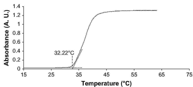
Fig. 3. Cloud point curve for PNIPAM ( M_n = 4500 ) in aqueous solution (2 mg/mL) at 500 nm with a heating rate of 1.4 °C/min.
