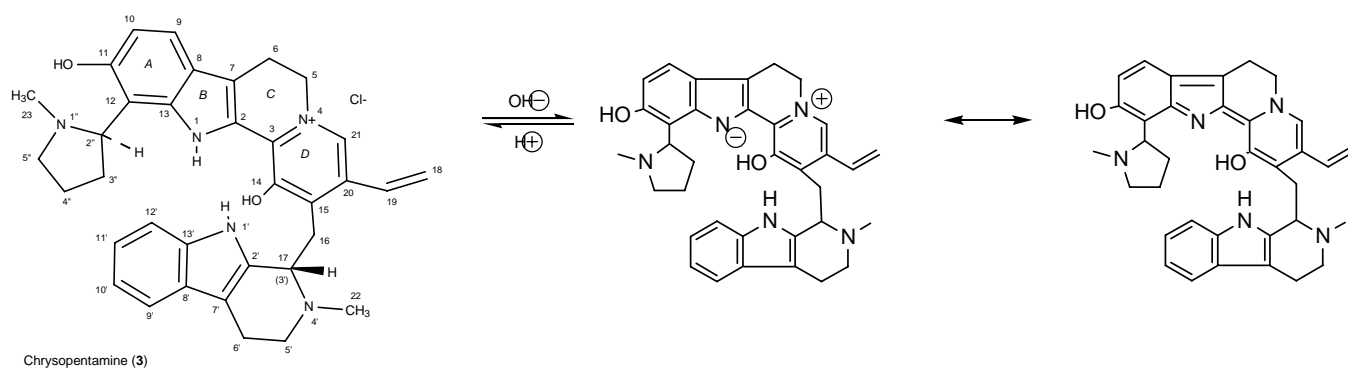
Chrysopentamine (3)
