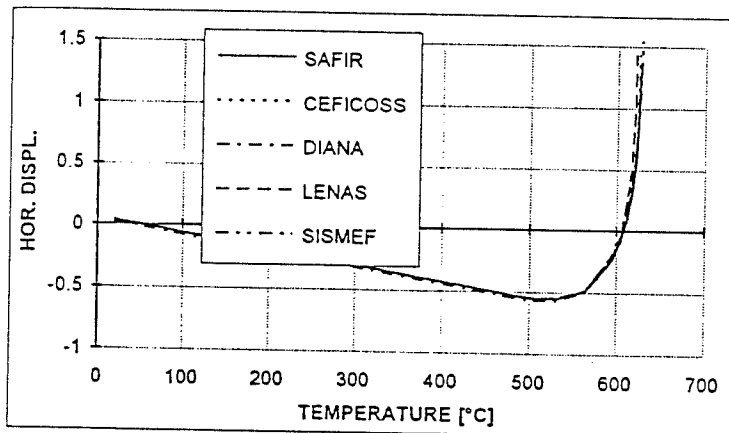
FIGURE 3. Lee's frame under uniformly increasing temperature.
