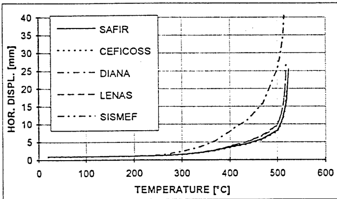
FIGURE 8. Centrally loaded column under increasing uniform temperature.
