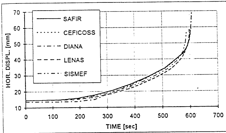
FIGURE 6. Eccentrically loaded column under ISO heating.
