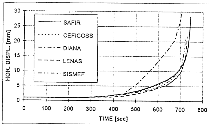
FIGURE 9. Eccentrically loaded column under ISO heating.
