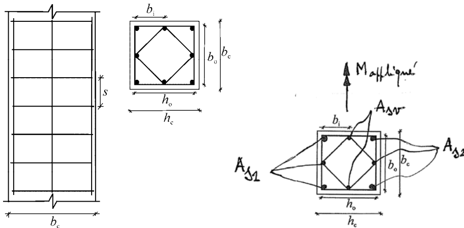
Figure 10.23. Armature de confinement.
