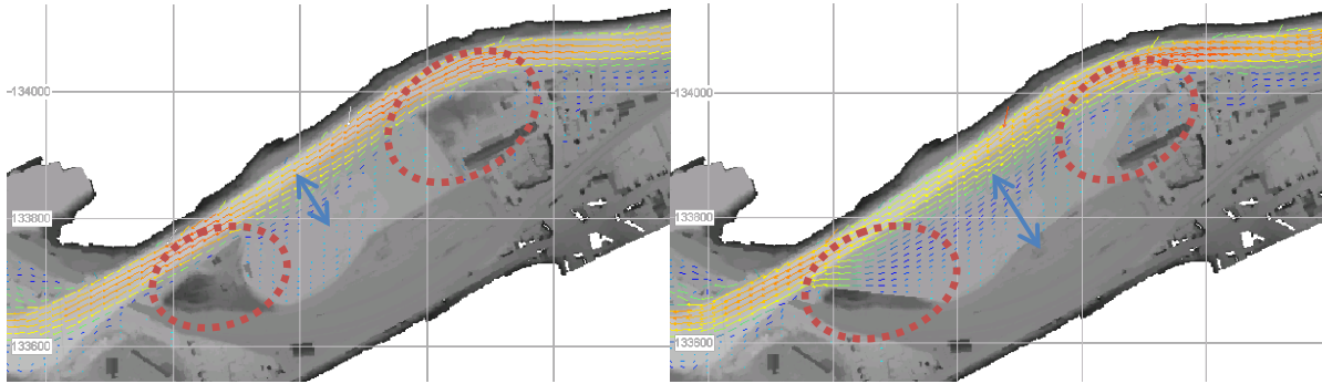
Figure 17: Velocity field (colour) and topography (grey) in Poulseur (upstream part of the case study of the river Ourthe). (a) situation without floodplain activation; (b) floodplain activation.
