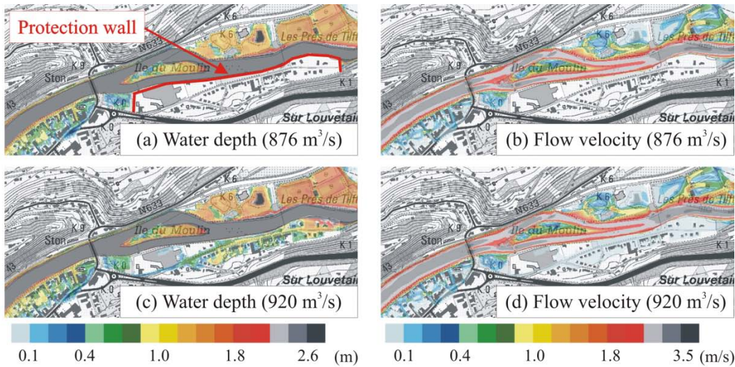
Figure 10: Water depth and flow velocity magnitude simulated for discharges just below (876m³/s) and just above (920m³/s) the threshold discharge for overtopping of the existing protection wall (flow from left to right).
