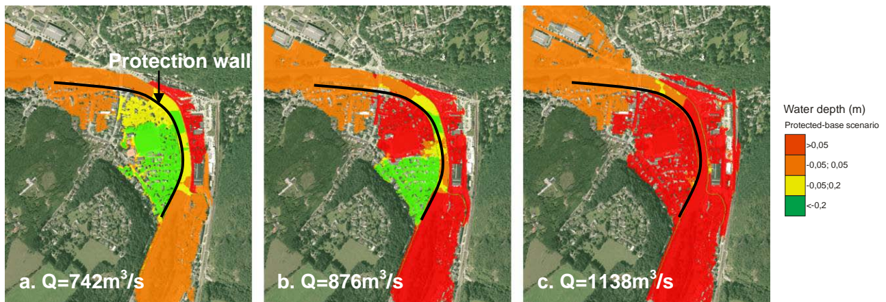
Figure 16: Sketch of the water depth differential between base and protected scenarios for three representative discharges for the wall heightening protection measure.
