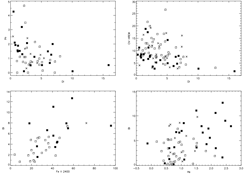
Fig. 1. The most significant non-trivial correlations (see text). p_0 is the debiased broad-band optical polarization (in %), DI is the detachment index (unitless), CIV HREW is the rest equivalent width of the red part of the CIV BEL (in Å), BI is the balnicity index (in 10^3 \text{ km s}^{-1} ), \alpha_B is the slope of the continuum measured shortward of C III] (unitless) and Fe II 2400 is the rest equivalent width of the Fe II emission feature near 2400 Å. Open squares are HI BAL QSOs, filled squares are LI BAL QSOs and crosses are unclassified BAL QSOs.
