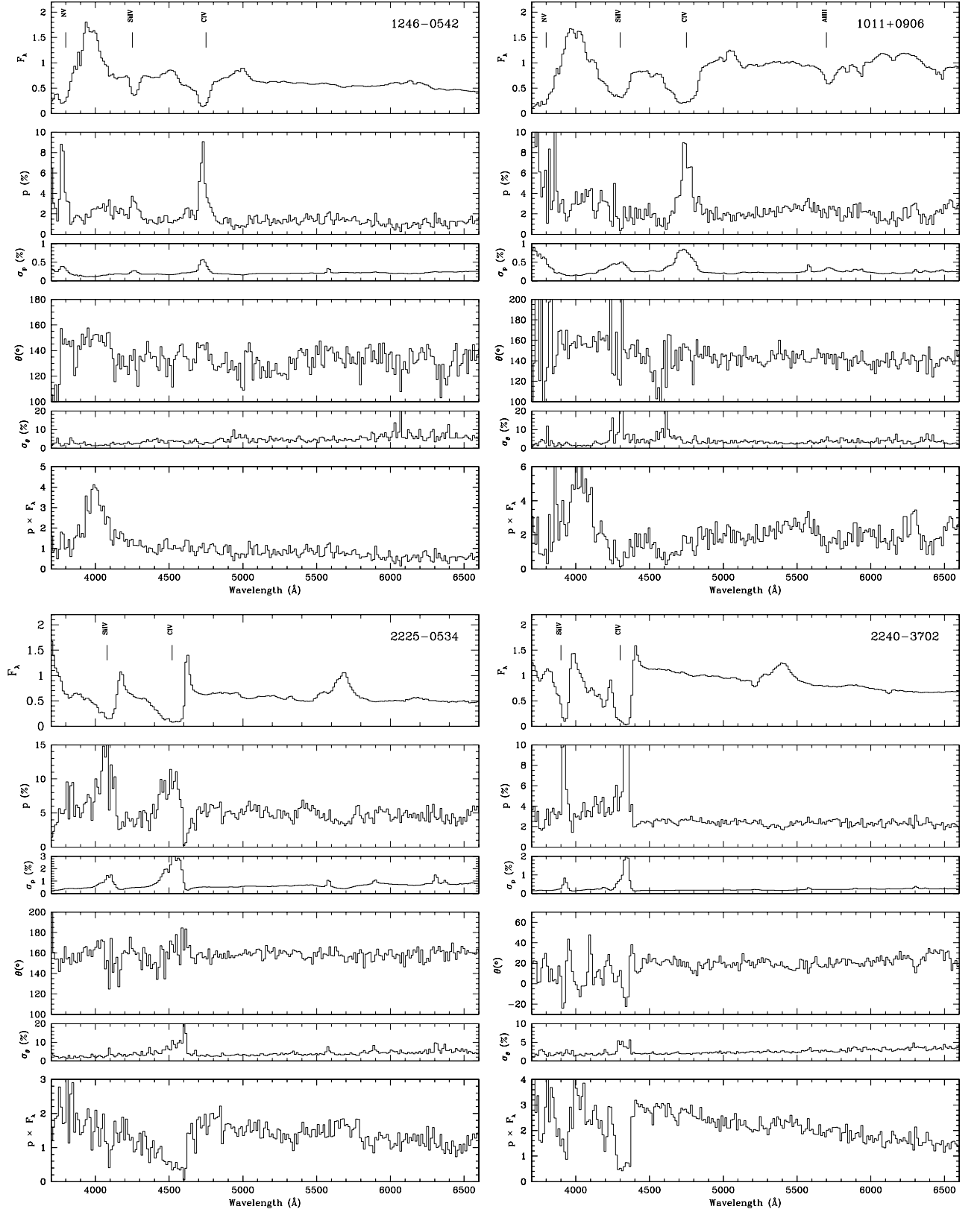
Fig. 3. Spectropolarimetric data for the BAL QSOs B1246–0542 ( top left ), B1011+0906 ( top right ), B2225–0534 ( bottom left ) and B2240–3702 ( bottom right ). For each object, there are six panels; from top to bottom : total flux F_\lambda , degree of polarization p , associated error \sigma_p , polarization position angle \theta , associated error \sigma_\theta , and polarized flux p \times F_\lambda . p has not been debiased. The main absorption lines are indicated.
