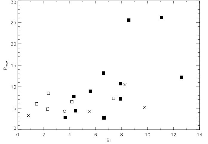
Fig. 5. The correlation between the maximum value of the polarization in the C IV absorption line and the balnicity index BI. Open squares are HIBAL QSOs, filled squares are LIBAL QSOs and crosses are unclassified BAL QSOs. The open circle corresponds to an uncertain measurement (see text).
