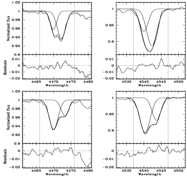
Fig. 1. Results of the fit of two Gaussians to the He I \lambda 4471 (left) and He II \lambda 4542 (right) lines for the spectra obtained on HJD 2 452 164.382 and HJD 2 452 922.388 respectively for the upper and lower figures. These profiles correspond respectively to phases 0.307 and 0.907 of our orbital solution. The individual components are overplotted. The vertical dashed lines give the boundaries of the domain where the fit was performed. The lower panels provide the residuals of the fit.
