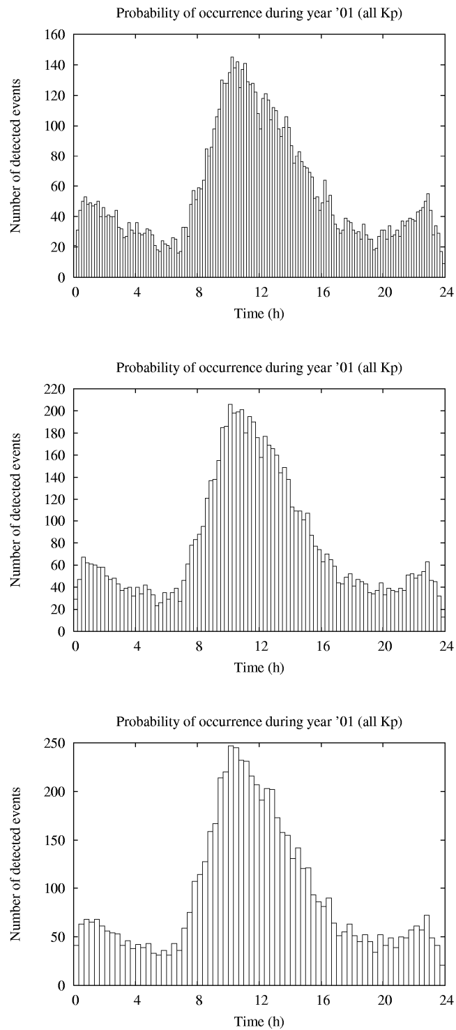
Figure 4.11 Number of ionospheric events detected at Brussels in 2001 in function of local time for time intervals of 10min (top), 15min (middle) and 20min (bottom).
