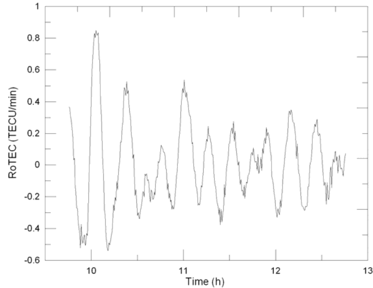
Figure 2.1. Vertical TEC variability (rate of change in TECU/min) due to a TID observed at Brussels along the track of satellite 7 on DOY 340 in 2001.
