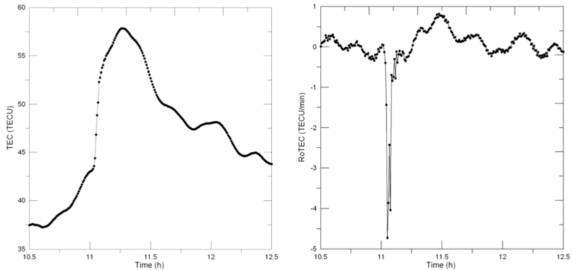
Figure 4.9 Effects of the solar flare of 28/10/03 on the TEC (left) and on the RoTEC (right) at Brussels (satellite 7).
