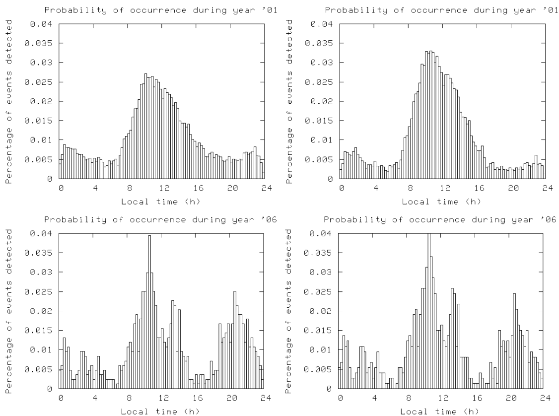
Figure 4.8 Ionospheric events distribution at Brussels for year 2001 (top) and 2006 (bottom) if we include (left) or not (right) the days which present Kp_{daily\ max} > 5 .
