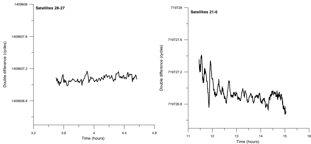
Figure 5.7 Double difference of the L1 phase (in L1 cycles) on DOY 359 in 2004, baseline Brussels-Saint Gilles (4 km), satellite pair 28-27 (left) and satellite pair 21-6 (right).
