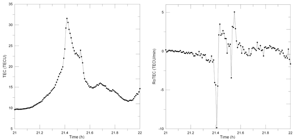
Figure 4.10 Effects of the geomagnetic storm of 30/10/03 on the TEC (left) and on the RoTEC (right) at Brussels (satellite 31).
