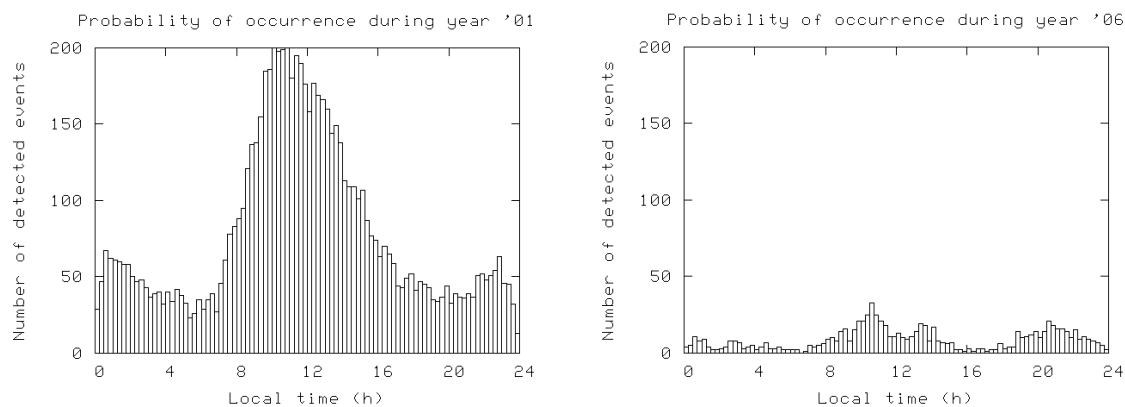
Figure 4.4 Ionospheric event distribution at Brussels for the year 2001 (solar maximum) and the year 2006 (solar minimum) in function of local time.
