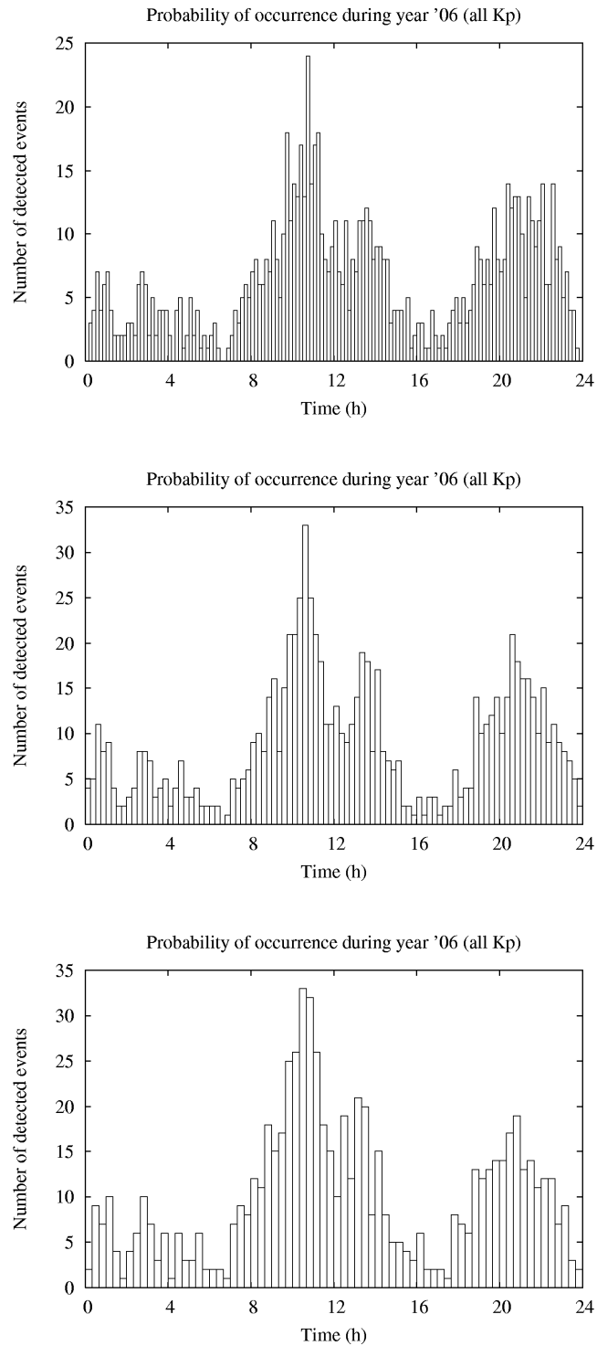
Figure 4.12 Number of ionospheric events detected at Brussels in 2006 in function of local time for time intervals of 10min (top), 15min (middle) and 20min (bottom).
