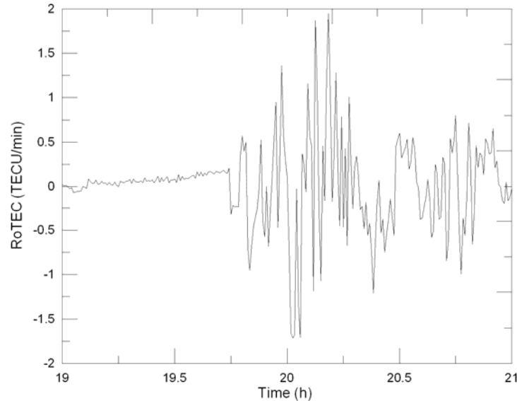
Figure 2.2. Noise-like variability in vertical TEC rate of change (in TECU/min) observed at Brussels during a geomagnetic storm on November 20 2002 along the track of satellite 22.
