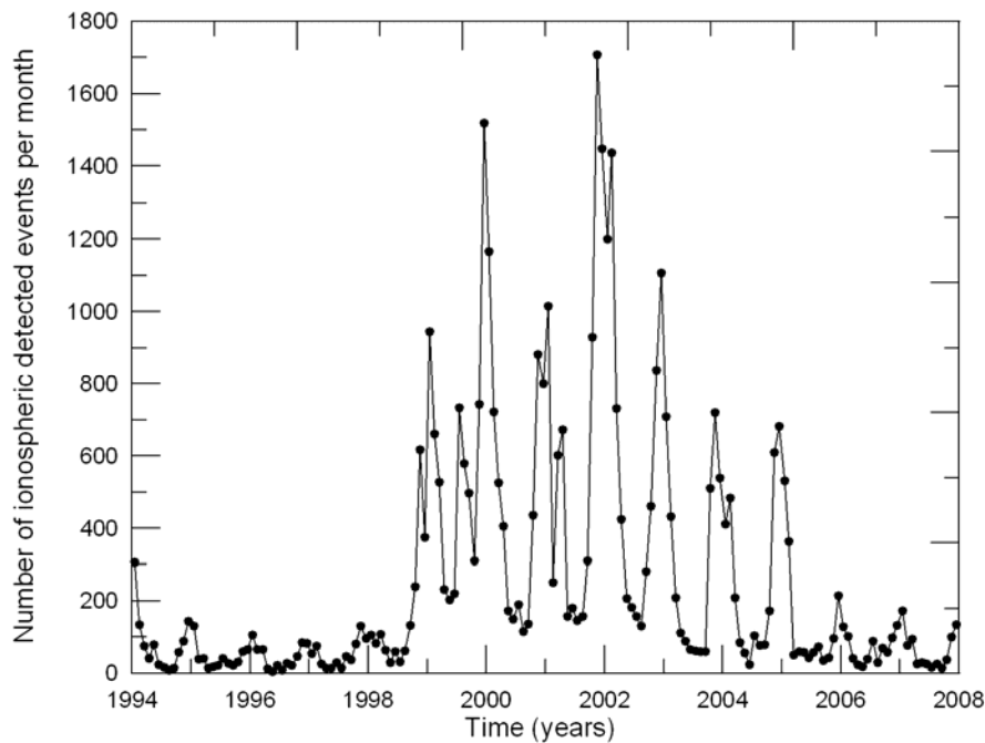
Figure 4.1 Number of detected ionospheric events per month at Brussels from January 1994 to December 2007.
