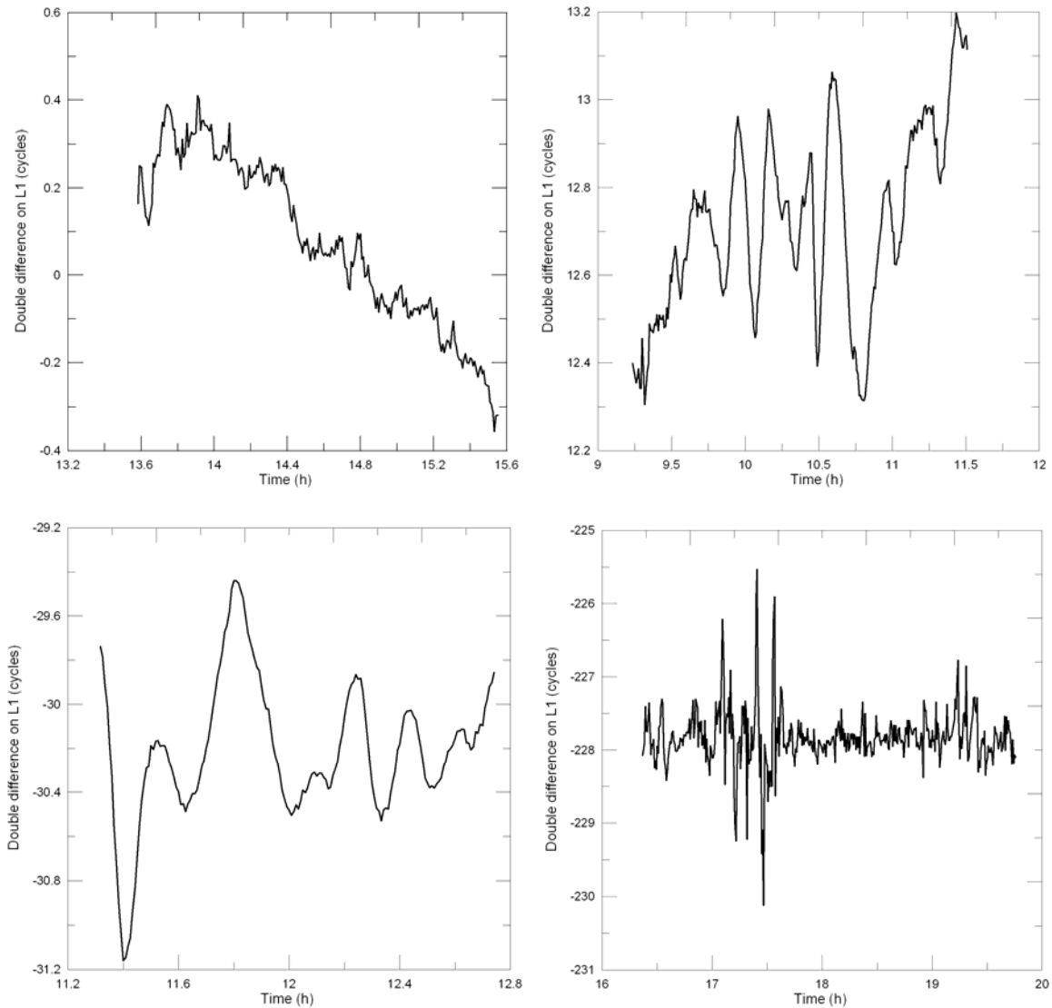
Figure 5.8 Double differences of the L1 carrier for the baseline OUDE-ZWEV, on DOY 103/07 satellite pair 23/2 (top left), DOY 359/04 satellite pair 5/6 (top right), DOY 301/03 satellite pair 7/5 (bottom left) and DOY 324/03 satellite pair 16/2 (bottom right).
