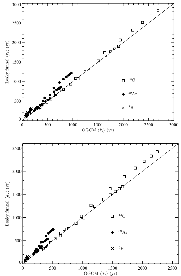
Fig. 4. Scatter plot of the predicted domain-averaged radioages (top) and radioactive tracer ages (bottom) versus those computed from the 3-D model. The leaky funnel ages are computed by means of eqs (31)–(32) and the parameters in Table 3. The linear correlation coefficients and rms differences corresponding to the fit for each of the radioactive tracer are given in Table 4.
