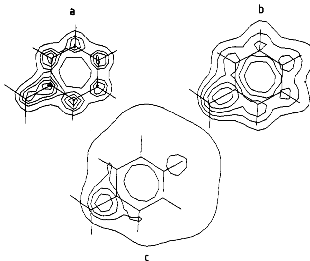
Figure 5. 2D TEH map for nitrobenzene within MINI-1 in the plane (a) Y = 1.2 \text{ \AA} , with contours at -115, -110, -100, -90, -80, and -60 \text{ kcal/mol} ; (b) Y = 1.6 \text{ \AA} , with contours at -40, -35, -30, -25, and -20 \text{ kcal/mol} ; (c) Y = 2 \text{ \AA} , with contours at -19, -17, -15, and -10 \text{ kcal/mol} .
