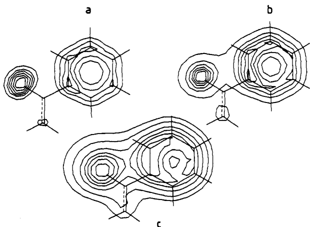
Figure 4. 2D TP maps for benzamide within the 6-31G** basis set in the plane (a) Y = 1.2 \text{ \AA} , with contours at -100, -95, -90, -85, -80, and -70 \text{ kcal/mol} ; (b) Y = 1.6 \text{ \AA} , with contours at -62, -60, -58, -55, -50, and -40 \text{ kcal/mol} ; (c) Y = 2 \text{ \AA} , with contours at -39, -37, -35, -33, -30, -25, and -20 \text{ kcal/mol} .
