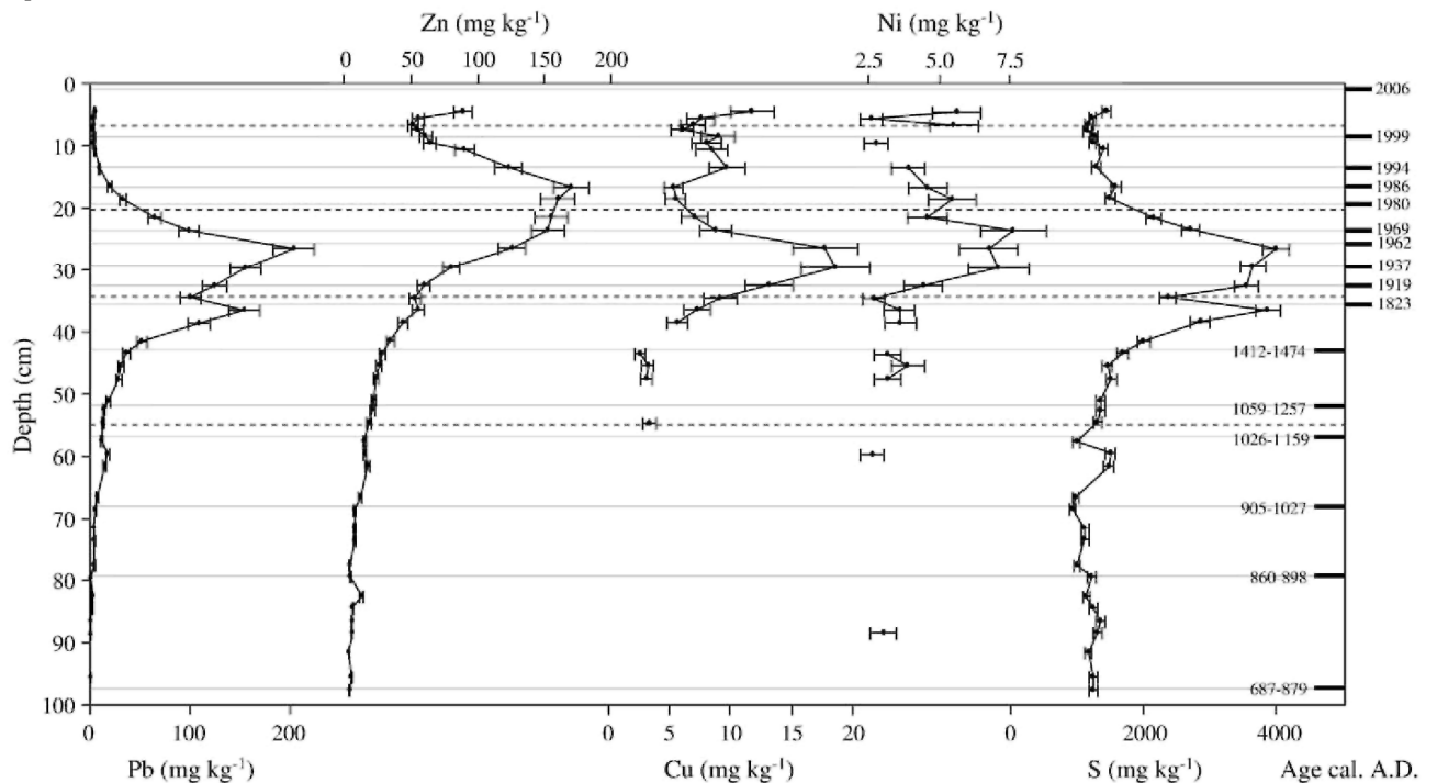
Fig. 2. [Pb], [Zn], [Cu], [Ni] and [S] vs depth. {}^{14}\text{C} age intervals and some {}^{210}\text{Pb} reference points are also reported.
