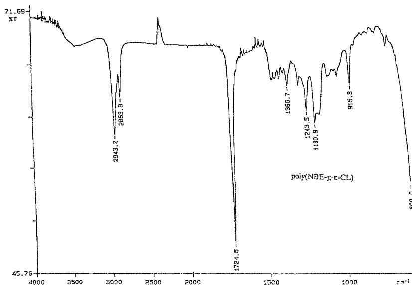
Fig. 3. FTIR spectrum of poly(norbornene-g-ε-caprolactone).
