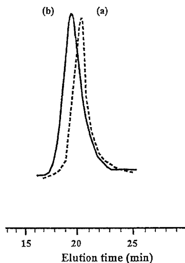
Fig. 2. Comparison of SEC traces for (a) polyCNBE-co-NBE-OH and (b) poly(norbornene-graft- \epsilon -caprolactone) (5 wt%NBE-OH).
