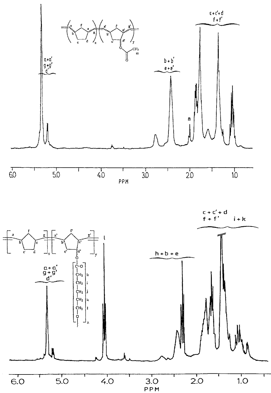
Fig. 1. ^1\text{H} NMR spectra ( \text{CDCl}_3 , TMS) of (a) poly(NBE-co-NBE-OAc) (3mol% NBE-OAc) and (b) poly(norbornene-g- \epsilon -caprolactone).
