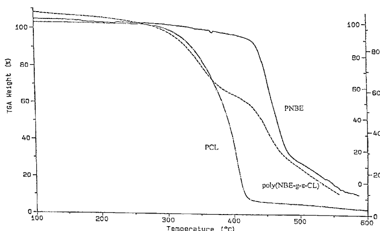
Fig. 5. Comparison of TGA traces for poly(NBE-g-ε-CL), PNBE and PCL.
