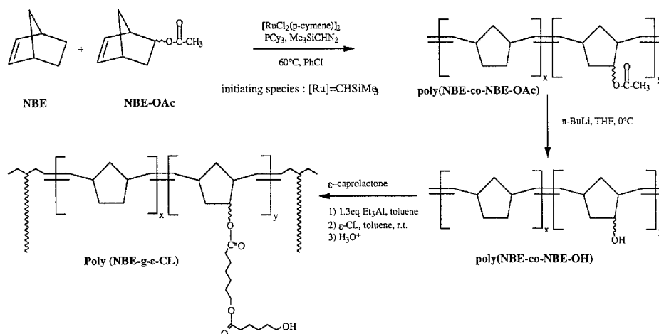
Scheme 1. Synthesis of poly(norbornene-g- \epsilon -caprolactone) by the "grafting from" strategy.
