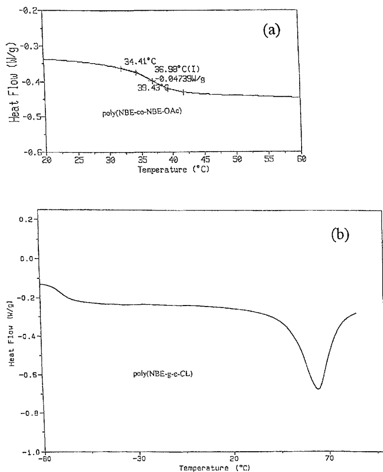
Fig. 4. DSC traces of (a) poly(NBE-co-NBE-OAc) (3 mol% NBE-OAc) and (b) poly(norbornene-
