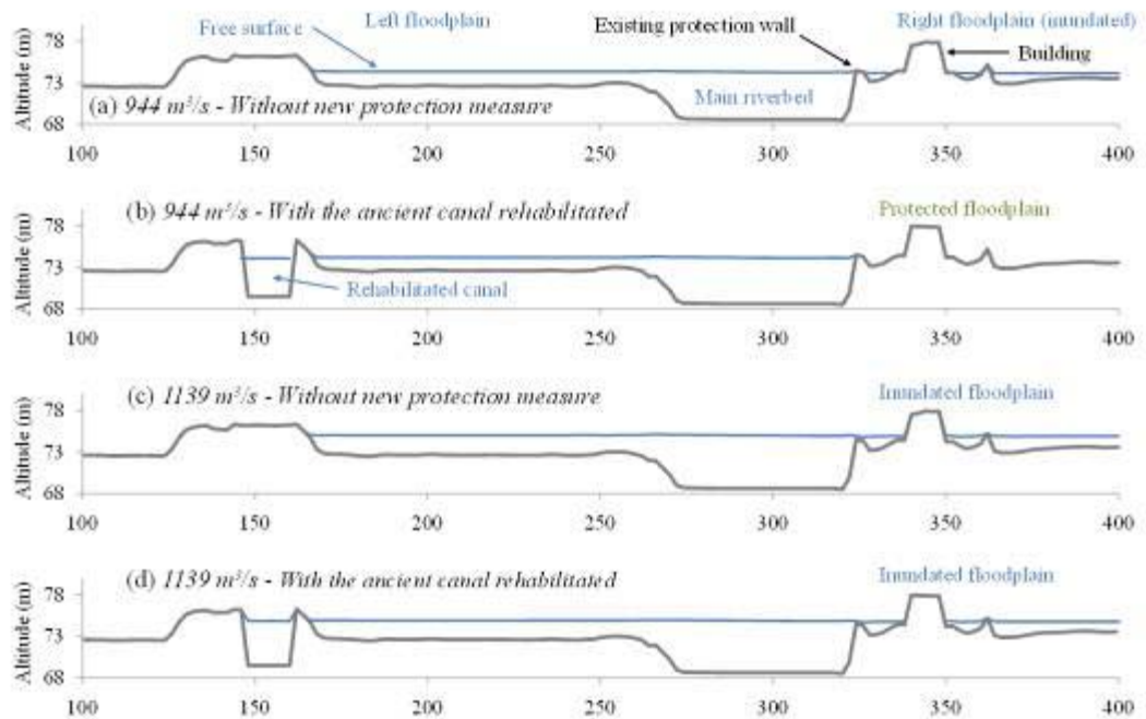
Figure 13. Typical cross-section (—) of river Ourthe in the case study area as well as corresponding free surface (—) for two different discharges (a, b: 944\text{m}^3/\text{s} ; c, d: 1139\text{m}^3/\text{s} ) in the present situation (a, c) and considering the ancient canal rehabilitated (b, d).
