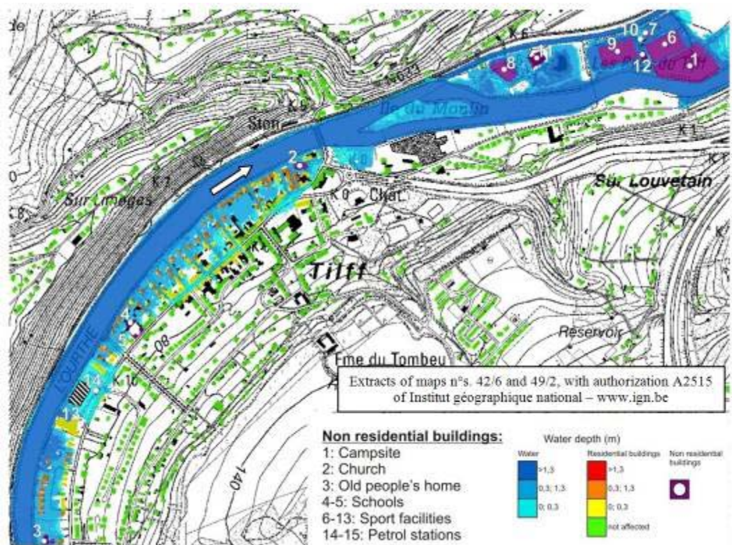
Figure 15. Spatial distribution of inundation depth (m, blue colour scale) and exposure of residential and non residential buildings (yellow to red colour scale), for a 154-year flood and considering the rehabilitation of the ancient canal.
