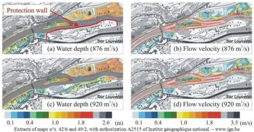
Figure 5. Water depth and flow velocity magnitude simulated for discharges just below (876m³/s) and just above (920m³/s) the threshold discharge for overtopping of the existing protection wall.
