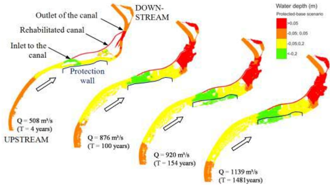
Figure 14. Difference in water depth (m) between the scenario with the ancient canal rehabilitated and the base scenario.
