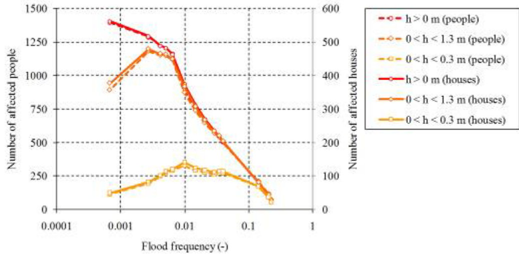
Figure 7. Exposure expressed by the number of affected people and flooded houses in the downstream reach of the case study, as a function of flood frequency.
