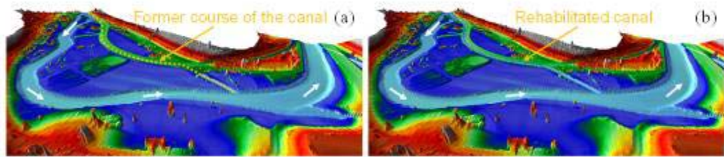
Figure 12. 3D view of the topography used for hydraulic modelling: (a) prior and (b) after rehabilitation of the ancient canal.
