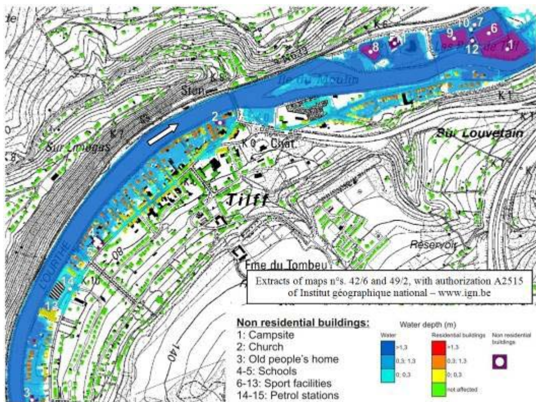
Figure 6. Spatial distribution of inundation depth (m, blue colour scale) and exposure of residential and non residential buildings (yellow to red colour scale), for a 154-year flood in the present situation.
