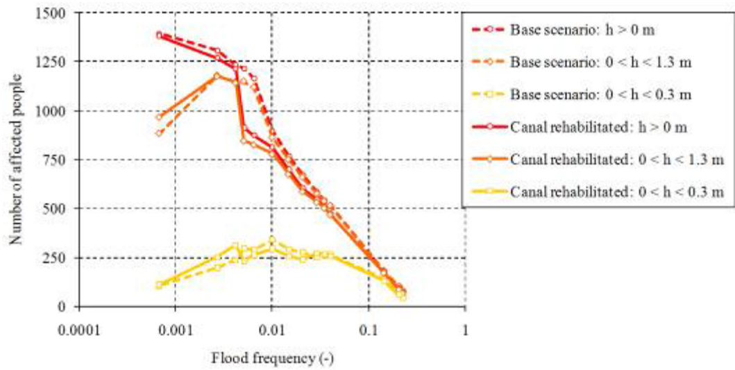
Figure 16. Influence of the rehabilitated ancient canal on the exposure, expressed as the number of affected people.
