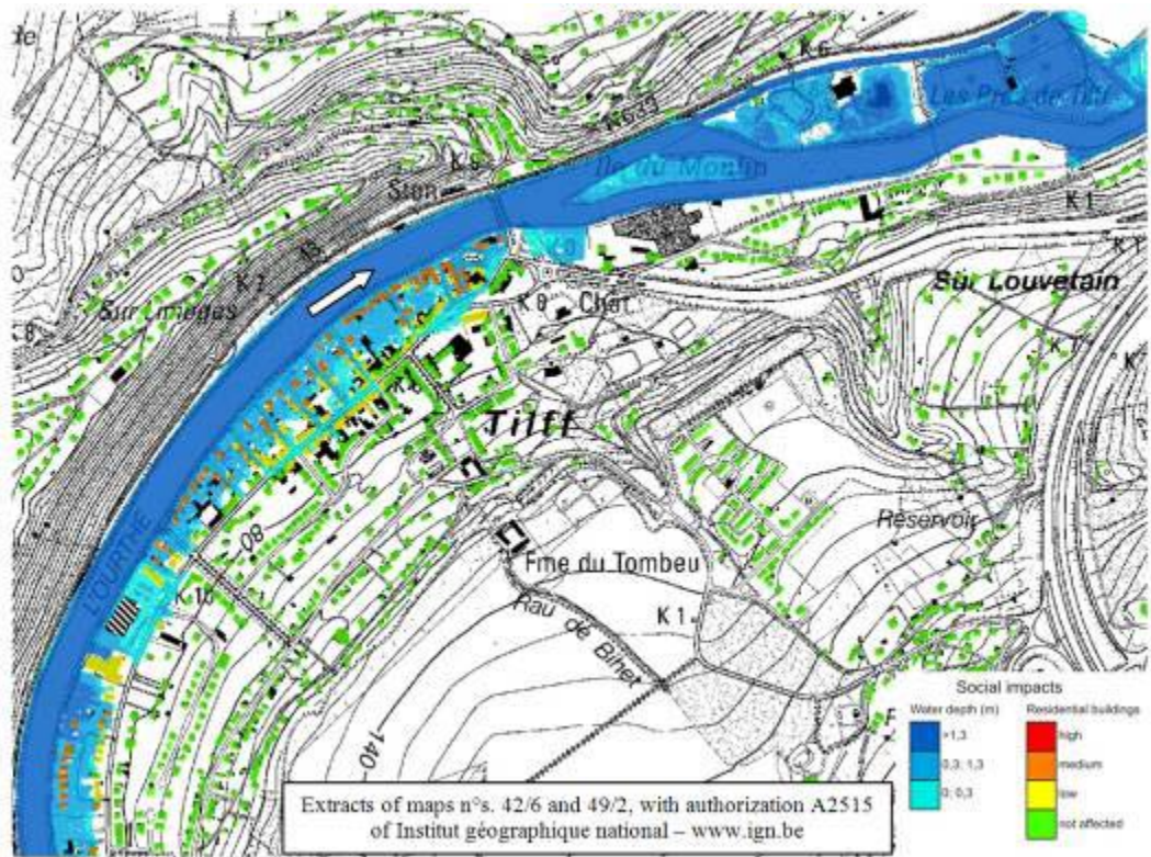
Figure 18. Spatial distribution of inundation depth (m, blue colour scale) and level of social impact (yellow to red colour scale), for a 154-year flood and considering the rehabilitation of the ancient canal.
