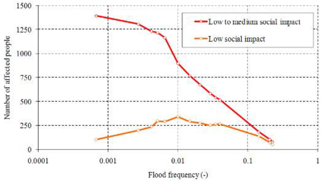
Figure 9. Social risk, expressed as the number of affected people in each category of social impact as a function of flood frequency (reach n°2 of the case study).
