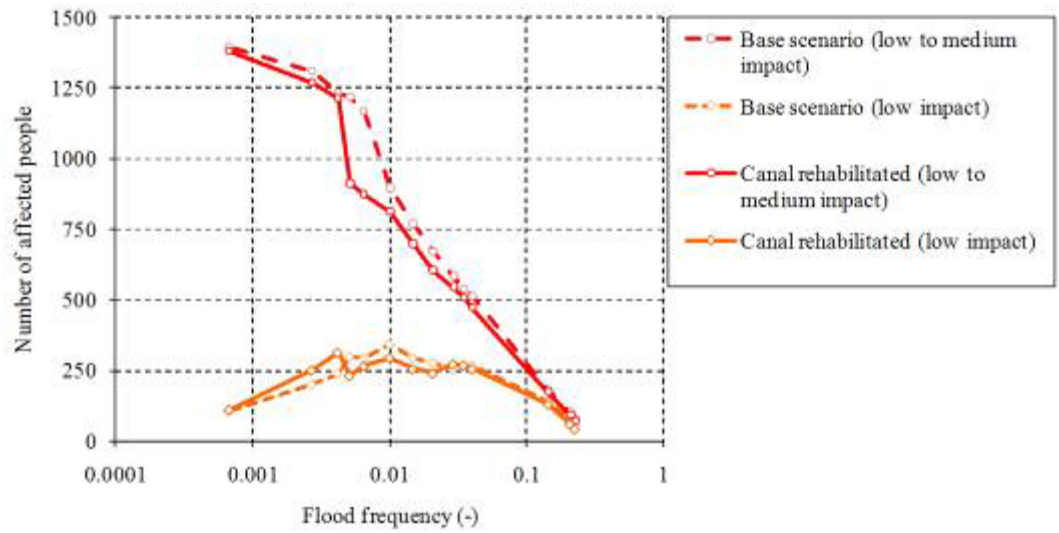
Figure 17. Influence of the rehabilitated ancient canal on the social risk curves.
