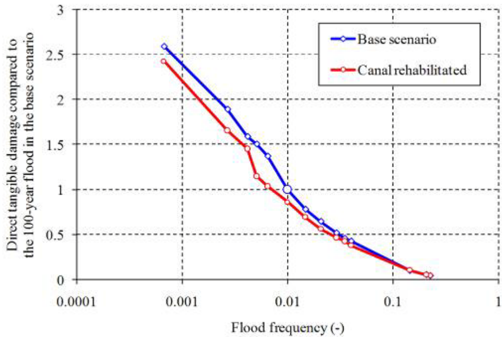
Figure 10. Economic risk curve for residential buildings, expressed by the direct economic damage compared to the direct economic damage for the 100-year flood (reach n°2 of the case study).
