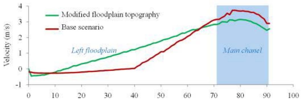
Figure 21. Cross-sectional distribution of flow velocity in the base scenario and considering a change in the topography of a floodplain in the upstream reach of the case study.
