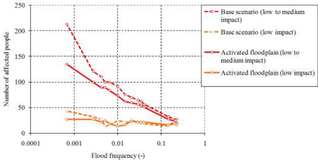
Figure 24. Influence of the activated passive floodplain on the social risk curve.
