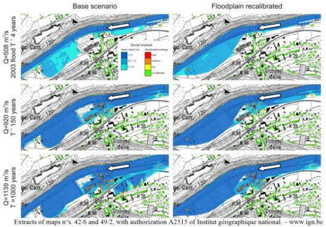
Figure 25. Spatial distribution of inundation depth (m) in the river and the floodplains (blue colour scale), as well as level of social impact (yellow to red colour scale).
