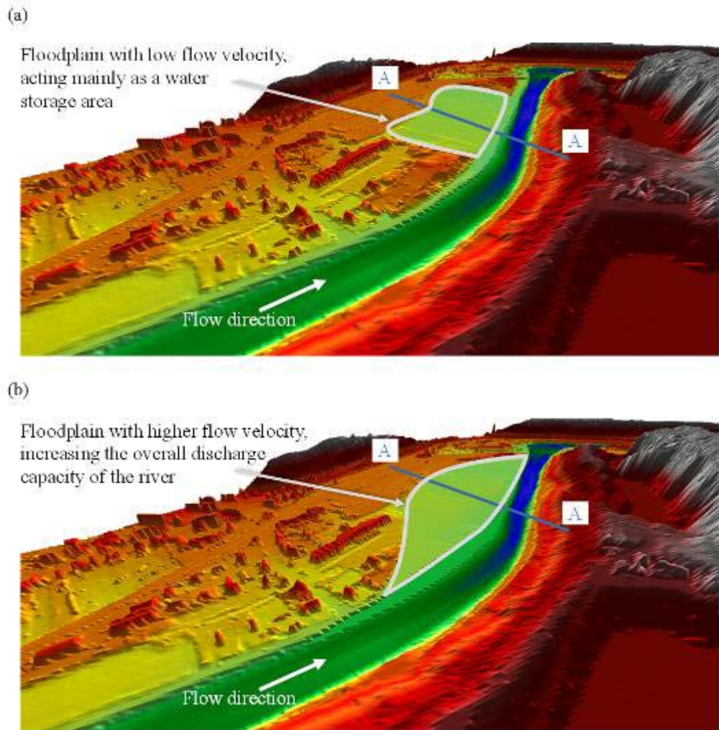
Figure 19. 3D view of topography in the upstream considered reach of river Ourthe, (a) in the base scenario and (b) after topography changes to increase discharge capacity in the left floodplain. The extent of the floodplain is highlighted in each figure, as well as cross-section AA for which velocity distribution is shown in Figure 21.
