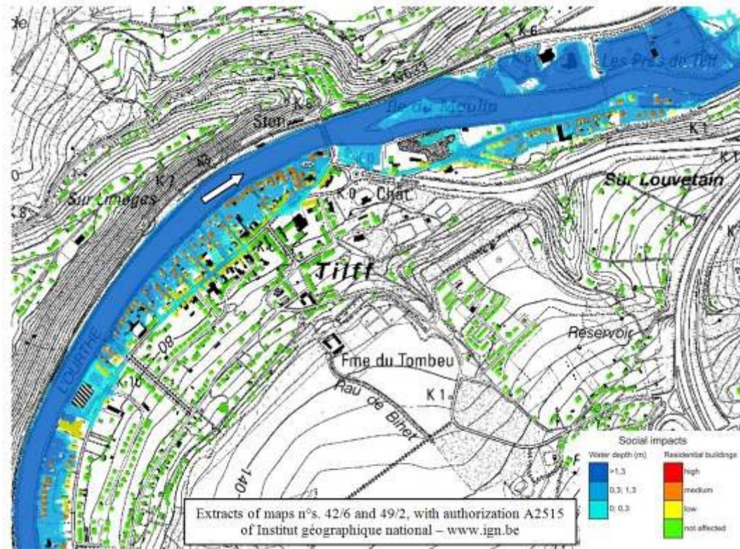
Figure 8. Spatial distribution of inundation depth (m, blue colour scale) and level of social impact (yellow to red colour scale) for a 154-year flood in the present situation.
