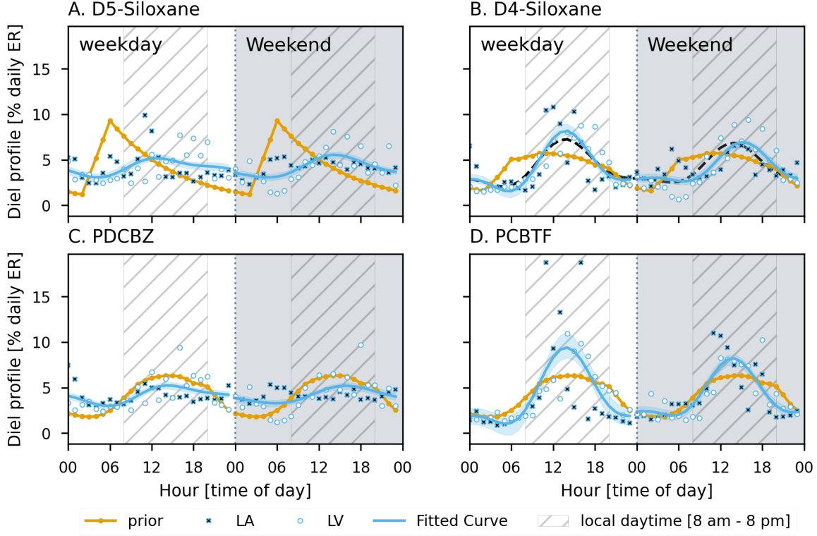
Figure 2: Diel profile (% of daily emission) as function of time of the day for D5-Siloxane, D4-Siloxane, PDCBZ, and PCBTF (A, B, C, and D respectively). White (gray) background denotes weekday (weekend) days for each tracer. Gray hatched regions denote local daytime (8 am to 8 pm). The orange curves are the prior for the area sources in the McDonald et al. inventory. Blue contoured black crosses (white dots) represent the inversion result for LV (LA) with second order Fourier sum (fitted to both) shown as a blue curve. The std range of the fitted curve are shown as blue shaded area behind the curve. The dashed line in panel B shows the diurnal emission profile for D4-Siloxane reconstructed by combining the other sub-sector optimized diel profiles.
