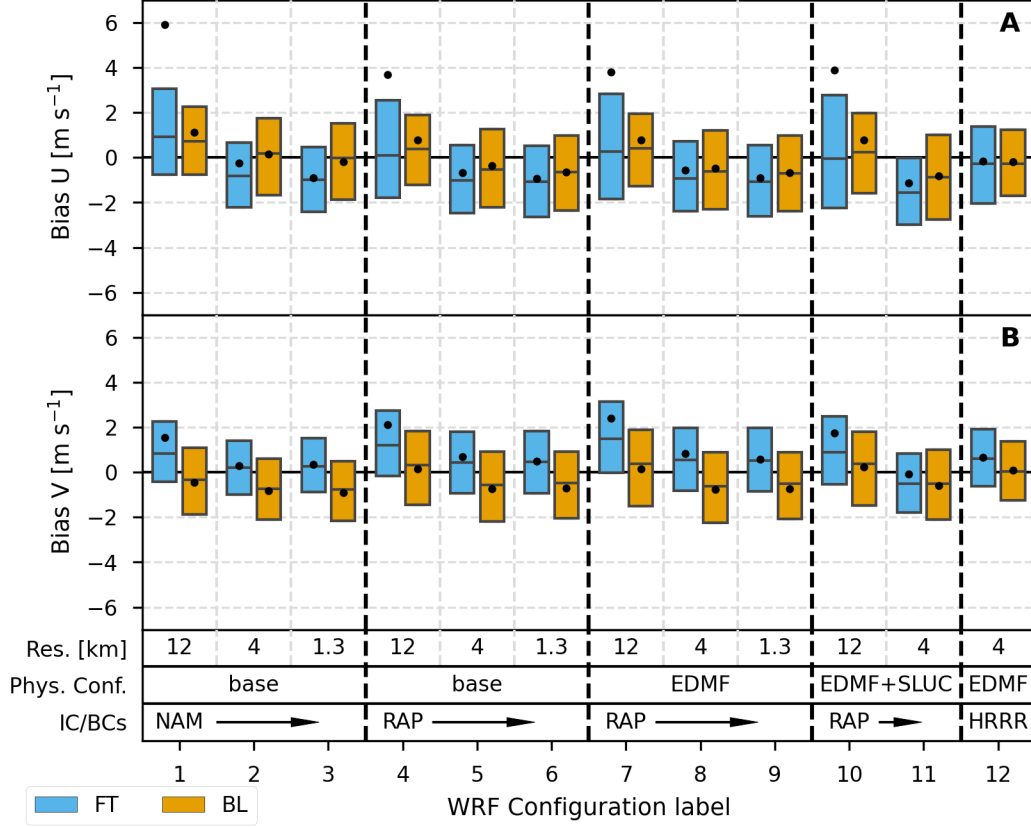
Figure 1: Biases in zonal (A) and meridional (B) wind directions for each WRF-Chem configuration using the mobile Doppler lidar observations as a reference. The boxes illustrate the median and the interquartile range of the biases for each data point in the observations, the average bias is represented by the black dot. Biases were separated by Free Troposphere (FT; blue), and Boundary Layer (BL; orange) regions according to model boundary layer height. The lowest three rows document the WRF-Chem configuration describing respectively (i) the model used to provide initial and boundary conditions (IC/BCs; nested runs represented by arrows), (ii) the PBL configuration, and (iii) the horizontal grid spacing.
