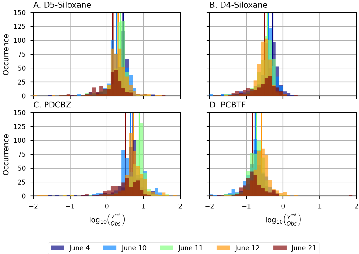
Figure 3: The distributions of the ratio between estimates combining the prior inventory with the calculated footprints ( y^{est} ) and the aircraft observations ( Obs ) for the VCP tracers (A, D5-Siloxane ; B, D4-Siloxane; C, PDCBZ; D, PCBTF). Distributions from each flight during RECAP-CA are shown and color-coded by flight. Median values are shown by the solid lines.
