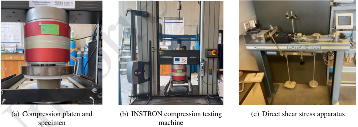
Figure 6. Testing equipment used for the unconfined compression and direct shear tests
