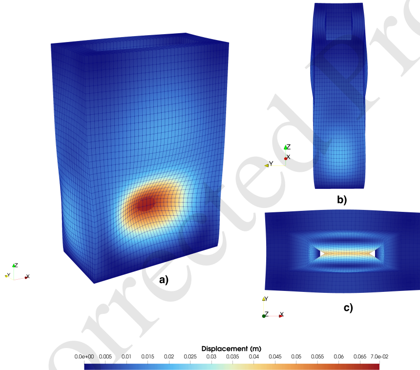
Figure 15. Displacement magnitude ( U , m) at the critical 37-layer height: isometric view (a), front view (b), and plan view (c)
