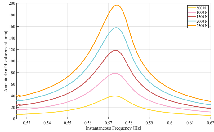
(a) Zoom on the envelope of the response of the structure excited by sine sweeps for lower amplitudes.
