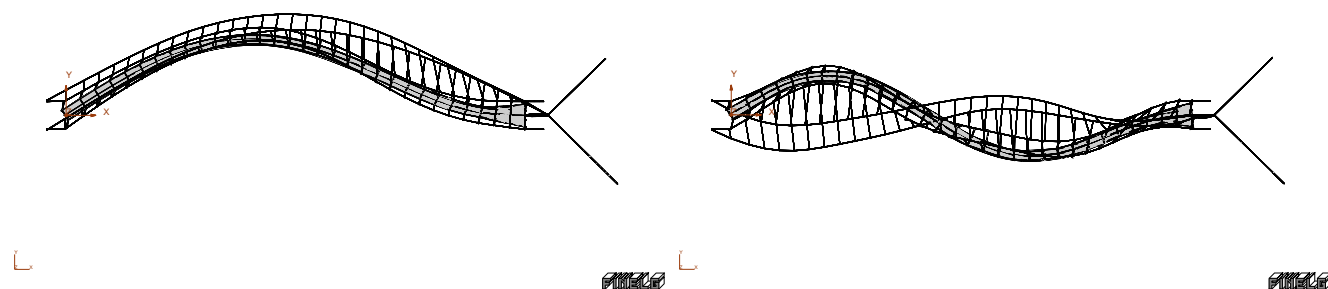
(a) Representation of the first horizontal eigenmode - f = 0.75 Hz - Amplification \times 25 . (b) Representation of the second horizontal eigenmode - f = 2.15 Hz - Amplification \times 25 .
