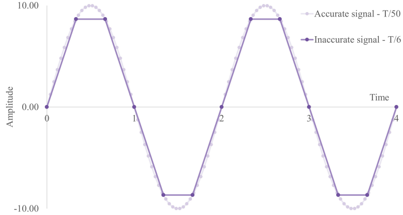
Figure 5.33: Example of distorted signal: the reconstruction of the signal never reaches the extrema of the sine.
