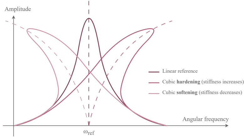
Figure 4.7: Evolution of the FRF based on the type of stiffness non-linearity.
