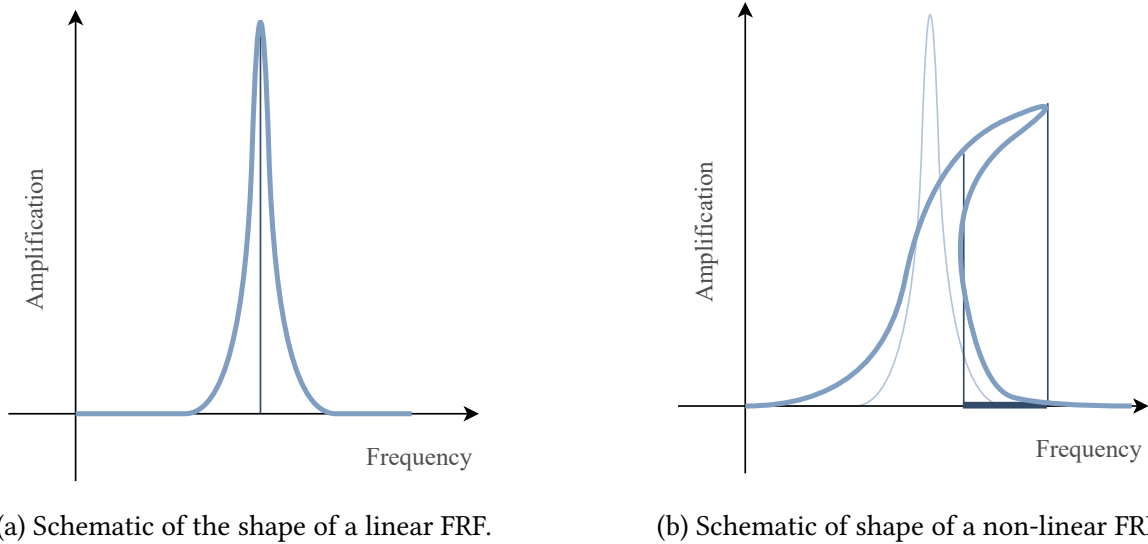
Figure 1.3: Schematic representation the difference of shape and amplification between a linear and non linear frequency response function.
