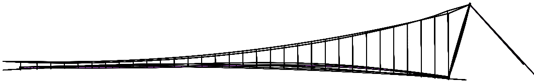
Figure 5.17: Updated deflection of the bridge, based on the residual stress distribution matching the hypothesis from the experimental campaign - amplified 2.5 times.
