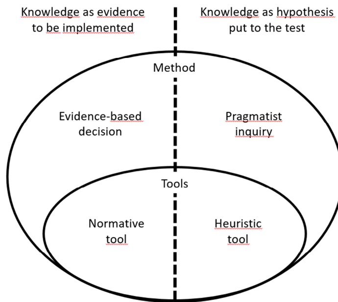
Figure 2: Analytical Framework.
