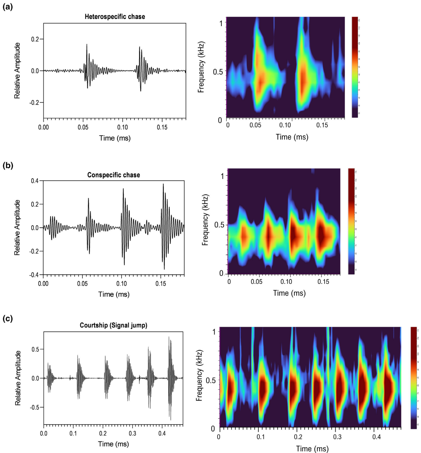
FIGURE 4 Oscillograms (left panels) and corresponding spectrograms (right panels) of sounds produced by Stegastes fuscus during heterospecific chasing (a), conspecific chasing (b) and courtship (signal jump) (c). Spectrograms were generated using a fast Fourier transform length of 512, Hann window and 50% overlap. Time is shown on the x-axis, and relative amplitude (oscillograms) or frequency (kHz; spectrograms) on the y-axis.
