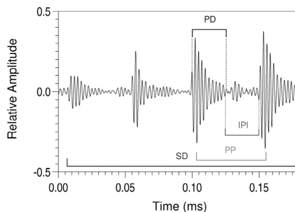
FIGURE 2 Oscillogram of a sound produced by Stegastes fuscus during conspecific chasing. The sound is composed of four pulses and illustrates sound duration (SD), pulse period (PP), pulse duration (PD), and interpulse interval (IPI).
