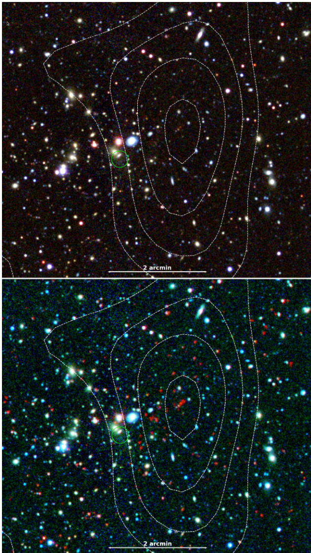
Figure 11. SPT-CL J2331-5736, the cluster with the highest redshift in SPTpol 100 d: The top image shows DES g , r , z colour composite image, and below is the DES g , r , and Spitzer ch1 colour composite image. The Spitzer image is taken from the SSDF (SPT Spitzer Deep Field). White contours show SPT-SZ S/N contours starting at 1 and increasing in steps of one. The green circle shows the location of a bright radio source detected in SUMSS. MCMF finds two counterparts, the high- z source visible only in the bottom image ( f_{\text{cont}} = 0.16 ) and the low- z cluster close to the radio source ( f_{\text{cont}} = 0.005 ).
