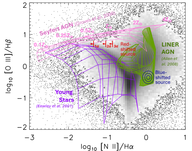
Figure 5. Line ratio diagram, comparing high-ionization [\text{O III}]/\text{H}\beta and low-ionization [\text{N II}]/\text{H}\alpha line ratios (J. A. Baldwin et al. 1981), which separates star-forming regions from active galactic nuclei and is insensitive to the effects of dust. The black/gray points in the background represent 85,224 galaxies with spectra from the Sloan Digital Sky Survey (L. J. Kewley et al. 2006). Where the point density becomes sufficiently high, we transition to a 2D histogram. There is a dense locus of points that are consistent with predictions for H II regions (L. J. Kewley et al. 2001) (purple grid). The blueshifted source on the western side of the stellar cavity has line ratios consistent with LINER AGN (T. M. Heckman 1980; M. G. Allen et al. 2008; green grid) and is inconsistent with models of star formation. The redshifted source on the eastern side of the stellar cavity has no detectable [\text{N II}] emission, and so appears here as an upper limit in [\text{N II}]/\text{H}\alpha . This source is fully consistent with models of Seyfert-like AGN with low-metallicity gas (B. A. Groves et al. 2006) (pink grid), but is also marginally consistent with a very young and energetic starburst. We rule out the latter scenario based on the lack of blue continuum emission, which would have been clearly visible in the archival HST data at F606W.
