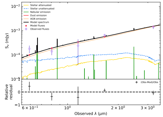
Figure A3. This figure, produced using the PCIGALE software (M. Boquien et al. 2019; G. Yang et al. 2022), shows the fluxes obtained for the central point source in each filter based on the two-dimensional image decomposition described in previous sections. This SED is well-described by a power law at all wavelengths. We model these data using PCIGALE, allowing for the combination of a two-stage star formation history, nebular emission, and an AGN, finding that the emission is best described by an AGN with contributions from nebular lines at the shortest wavelengths. The fact that these data are well-described by a single power law, despite being obtained over the course of 20 yr, suggests minimal time variability in the central point source.
