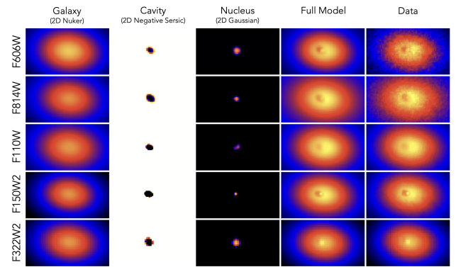
Figure A1. The surface photometry for the central galaxy in A402 has been modeled using a combination of a Nuker profile (A. W. Graham et al. 2003) for the “galaxy,” a negative-intensity Sérsic profile for the “cavity,” and a pointlike Gaussian for the “nucleus,” all convolved with the instrumental PSF. All models shown represent the average model fit when marginalizing over variations in the PSF and the count rate. The component models are shown without the PSF convolution applied, while the “full model” panels include the instrumental PSF. This figure demonstrates that the large variations in the observations can be attributed to a central AGN with a steep wavelength dependence and a PSF that is a factor of two larger at F110W and F322W2 compared to F606W, F814W, and F150W2. This image decomposition allows us to accurately measure the total flux missing in the cavity (Figure 2), the SED of the missing stars in the cavity and the galaxy (Figure A2), and the spectral energy distribution of the point source (Figure A3).
