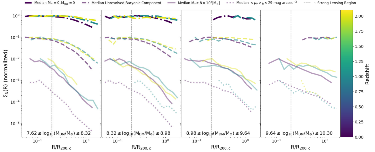
Figure 6. Median projected number density profiles of subhaloes along 36 different sightlines centred on our target clusters in TNG50 over time. For clarity, we show this for only z = 0, 1 , and 2 . The profiles have been arbitrarily normalized to highlight their differences in shape. Each panel represents a different mass bin as in Fig. 4. We can see, as expected, qualitatively flatter shapes, due to the effects of projection. Given the integrated nature of gravitational lensing, low-mass subhaloes both from the cluster itself and from the field are more likely to be found around the strong lensing region than suggested by the 3D profiles.
