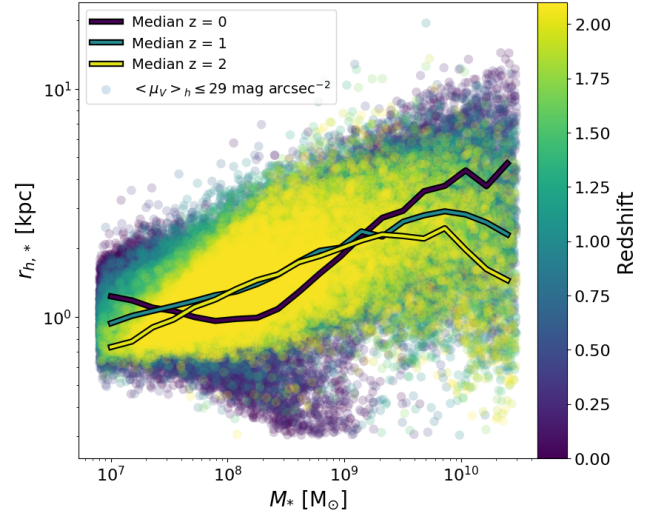
Figure 1. Stellar half-mass radius ( r_{h,*} ) as a function of stellar mass ( M_* ). Each point represents an object at the redshift indicated by the colour bar. Median lines are shown for redshifts 0, 1, and 2. We note the presence of a few extremely compact objects that reside in the field at z = 0 that pull the median line down in the range 10^8 \leq M_*/M_{\odot} \leq 10^9 . Taking that into account, we can see that the surface brightness cut of \langle \mu_V \rangle_h = 29 \text{ mag arcsec}^{-2} introduces a bias towards detecting only the more compact systems at fixed stellar mass for particularly low-mass galaxies.
