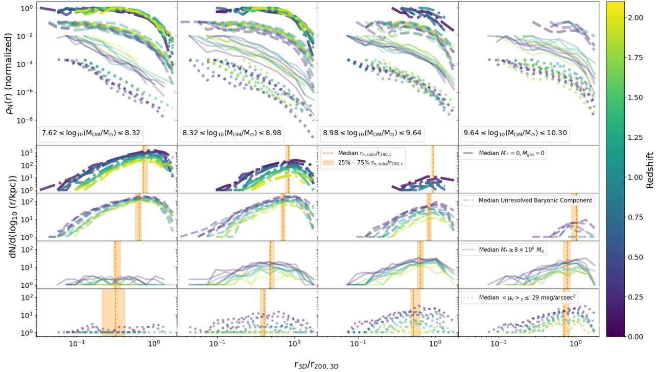
Figure 4. Top panels: The median number density profiles of subhaloes as a function of r/r_{200,c} in our targeted galaxy groups and clusters over time for subhaloes in the mass range 7.62 \leq \log_{10}(M_{DM}/M_{\odot}) \leq 8.32 (leftmost panel), 8.32 \leq \log_{10}(M_{DM}/M_{\odot}) \leq 8.98 (middle-left panel), 8.98 \leq \log_{10}(M_{DM}/M_{\odot}) \leq 9.64 (middle-right panel), and 9.64 \leq \log_{10}(M_{DM}/M_{\odot}) \leq 10.30 (rightmost panel). Lower panels: Number of subhaloes per \log_{10}(r/\text{kpc}) , dN/d\log_{10}(r) as a function of r/r_{200,c} for the same mass bins. Each lower panel shows a different component of subhaloes: M_* = 0 , M_{\text{gas}} = 0 (opaque dot-dashed lines coloured by redshift), those with an unresolved baryonic component (translucent dashed lines), those with M_* \geq 8 \times 10^6 M_{\odot} (transparent lines), and those with \langle \mu_V \rangle_h \leq 29 \text{ mag arcsec}^{-2} (translucent dotted lines). Each line in each panel represents the median value of the number (density) between the three target clusters at each radial bin at each redshift. For comparison, we show the median half-number radii and their 25–75 percentile spreads in the vertical orange dashed line and corresponding shaded region, respectively. We can see that while they have a greater half-number radius, dark and observationally dark subhaloes of mass \log_{10}(M_{DM}/M_{\odot}) \leq 8.98 are most likely, by number, to reside in the strong lensing region of our target groups and clusters at all redshifts.
