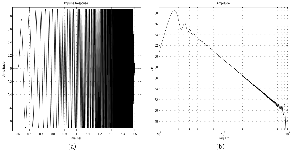
Figure 9: (a) Time representation of a Sine Sweep excitation signal ( \omega_1 = 2\pi 10 rad/s and \omega_2 = 2\pi 1000 rad/s). (b) Corresponding Magnitude spectrum.
