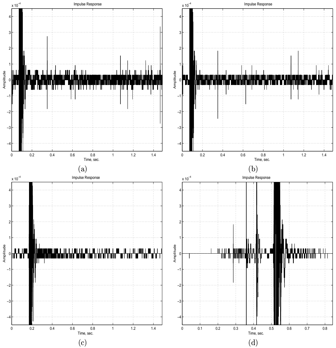
Figure 15: Zoom on the impulse responses obtained in the anechoic room with different methods. (a) MLS (b) IRS (c) Time-Stretched Pulses (d) SineSweep.
