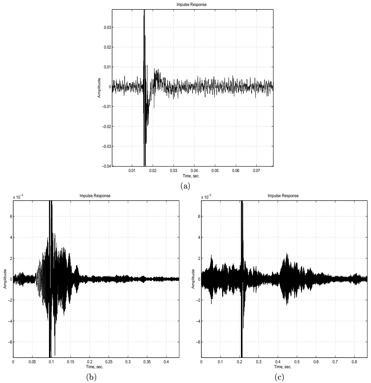
Figure 16: Impulse responses obtained in the anechoic room with different methods when an intense impulsive noise is simultaneously present. (a) MLS (b) Time-Stretched Pulses (c) SineSweep. Notice that the amplitude scales are not identical.
