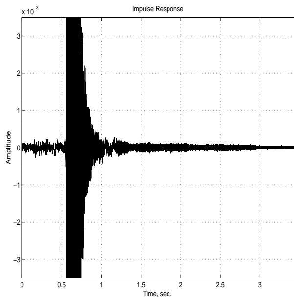
Figure 6: Zoom on the impulse response of a classroom obtained when a time-stretched pulse of about 6 seconds is used.
