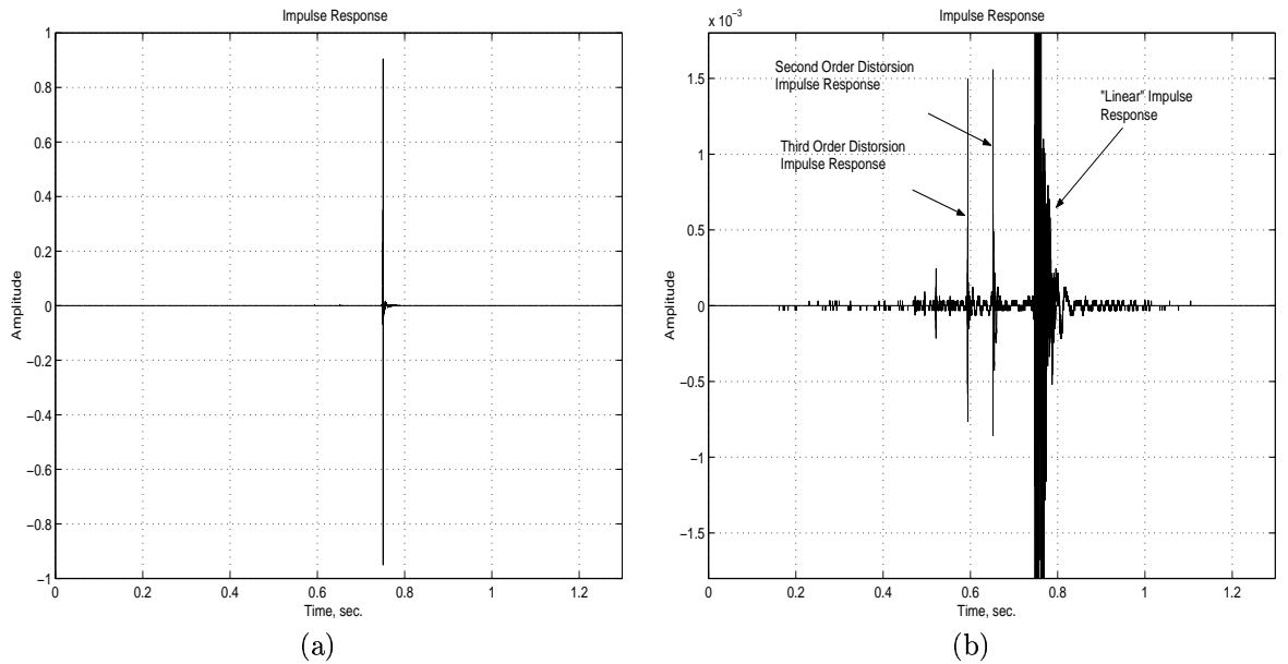
Figure 11: (a) Impulse Response obtained in an anechoic room with a logarithmic SineSweep of 1 second characterized by \omega_1 = 2\pi 10 rad/s and \omega_2 = 2\pi 22000 rad/s. (b) Zoom on this response showing the extraordinary precision of the achievable results.
