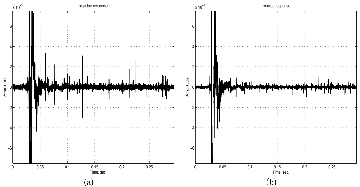
Figure 4: Zoom on the impulse responses obtained via MLS and IRS methods. (a) MLS method. (b) IRS method.
