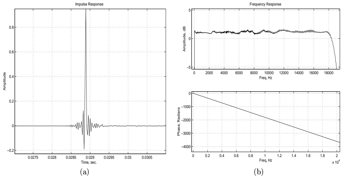
Figure 13: (a) Impulse response obtained in an anechoic room when the excitation signal has been preequalized (in this example, the Logarithmic SineSweep technique has been used). (b) Corresponding Magnitude and Phase Spectra.
