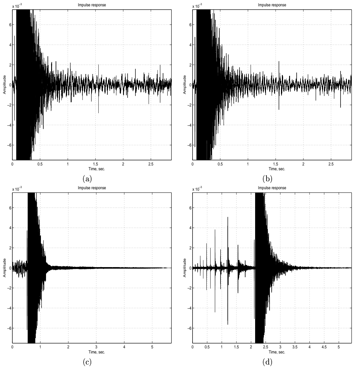
Figure 18: Zoom on the impulse responses obtained in the auditorium 604 of the Europe Amphitheater of the University of Liège (Belgium). (a) MLS (b) IRS (c) Time-Stretched Pulses (d) SineSweep.
