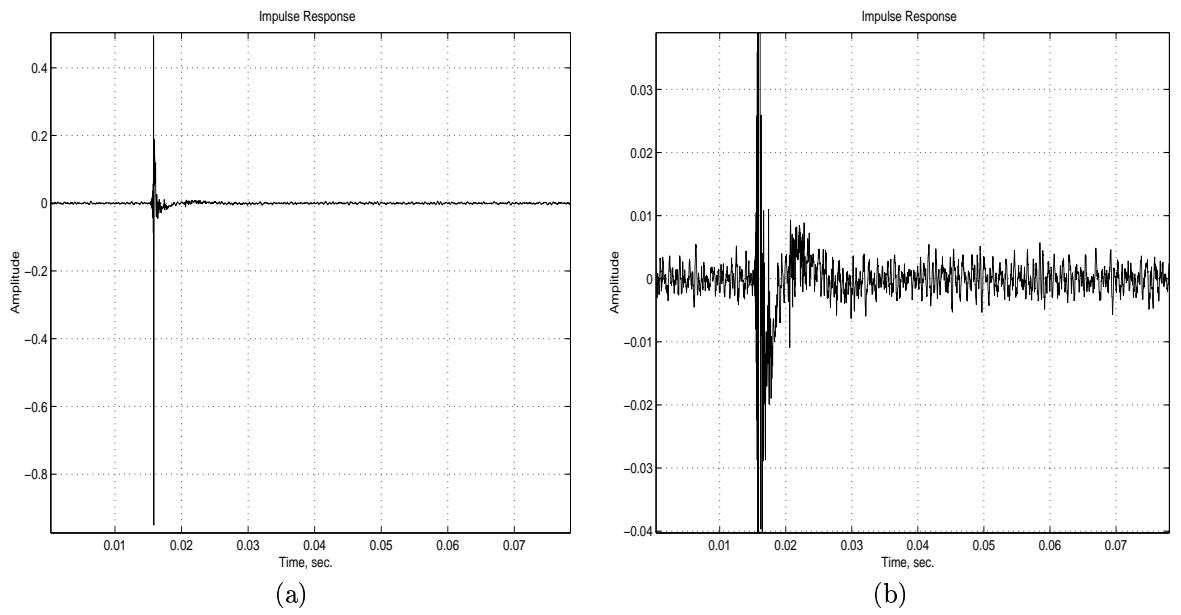
Figure 3: (a) Impulse response obtained with a single MLS sequence of order 16 in an anechoic room when Impulsive Noise is simultaneously present. (b) Zoom on the magnitude scale.
