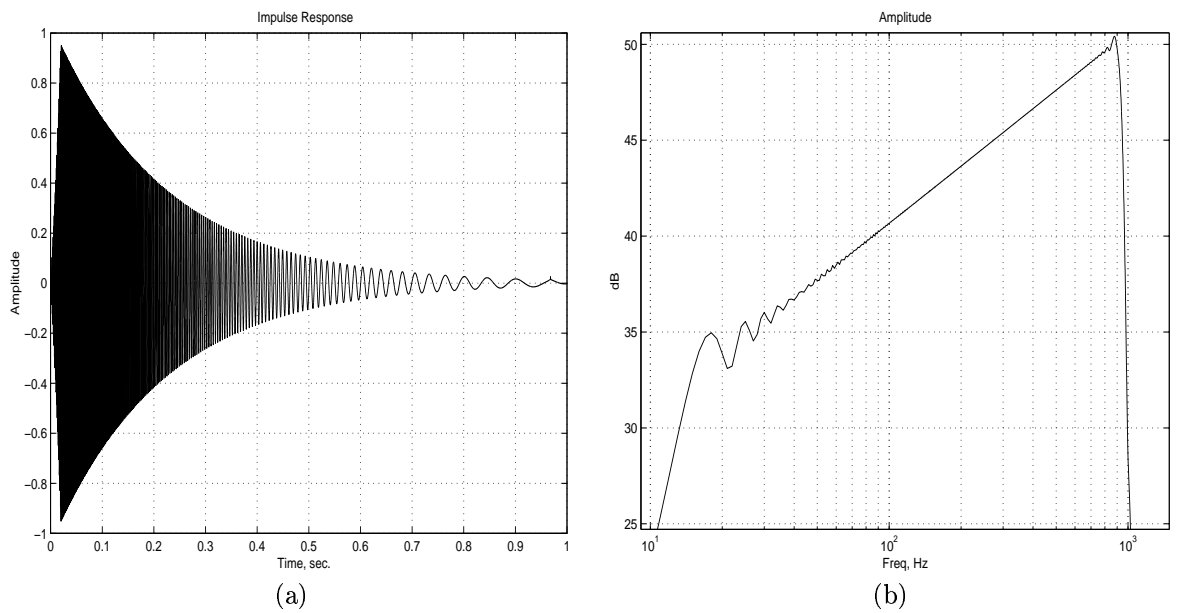
Figure 10: (a) Time representation of the inverse filter corresponding to the SineSweep signal presented in figure 9. (b) Corresponding Magnitude spectrum.
