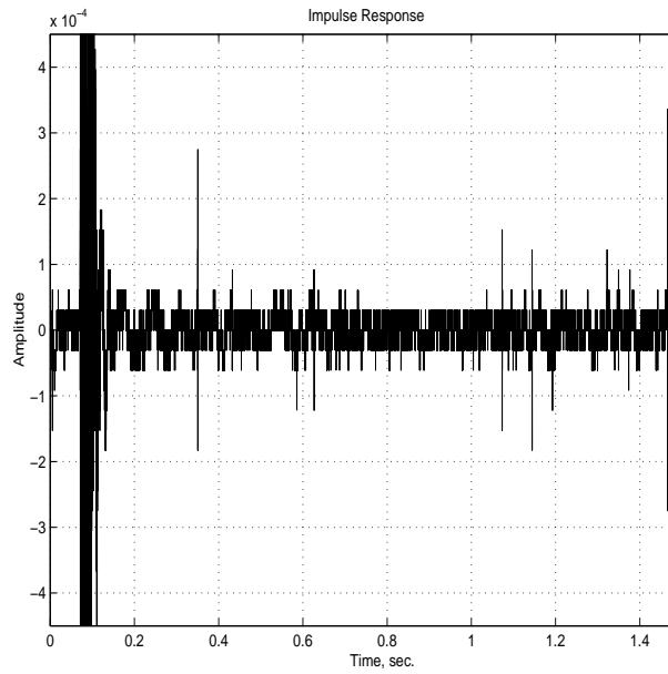
Figure 5: Zoom on the impulse response obtained when optimization of the measurement parameters (i.e. output sound level) of the MLS technique is realized .
