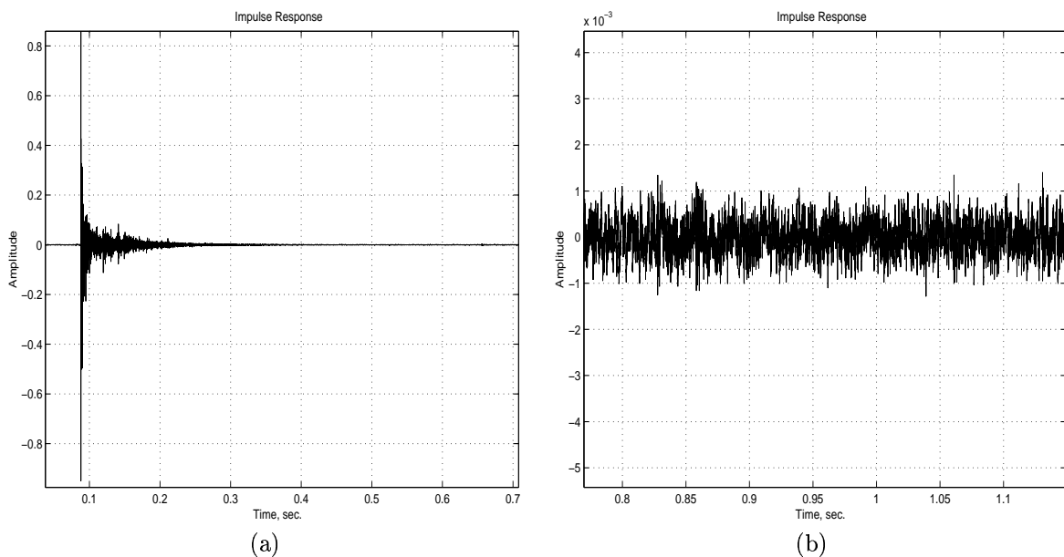
Figure 2: (a) Impulse response of a classroom obtained with a single MLS sequence of order 18 when a white noise generator is simultaneously present. The Noise Level measured at the position of the microphone is 60 dB. (b) Zoom on the end of the impulse response.
