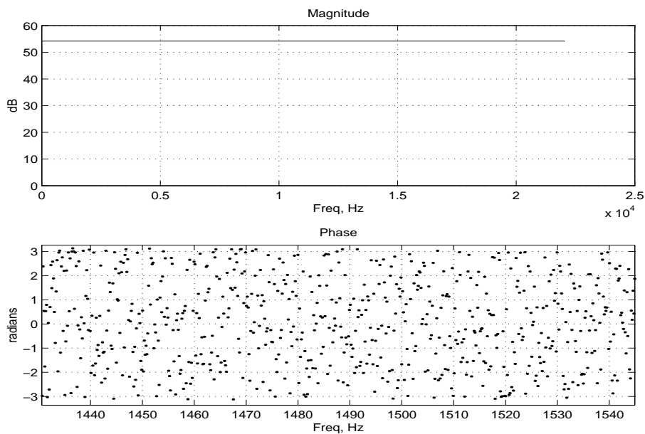
Figure 1: Magnitude and Phase Spectra of an MLS sequence. The phase spectrum has been enlarged in order to clearly show its uniform random distribution.
