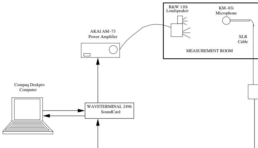
Figure 12: Schematic Representation of the measurement system.
