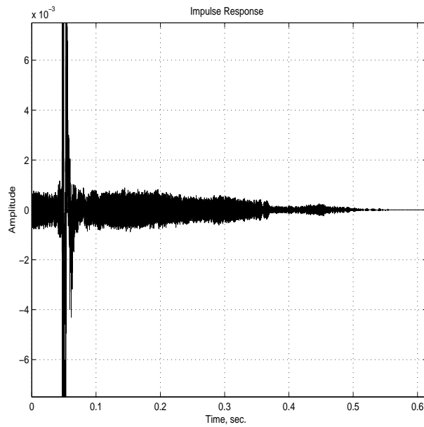
Figure 7: Zoom on the impulse response obtained in an anechoic room when a time-stretched pulse of about 1 second is used. In this case a bad quality loudspeaker has been used in order to emphasize the non linearity of the measurement system.
