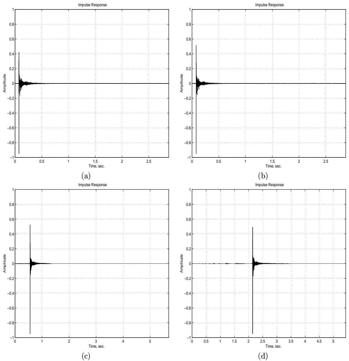
Figure 17: Impulse responses obtained in the auditorium 604 of the Europe Amphitheater of the University of Liège (Belgium). (a) MLS (b) IRS (c) Time-Stretched Pulses (d) SineSweep.
