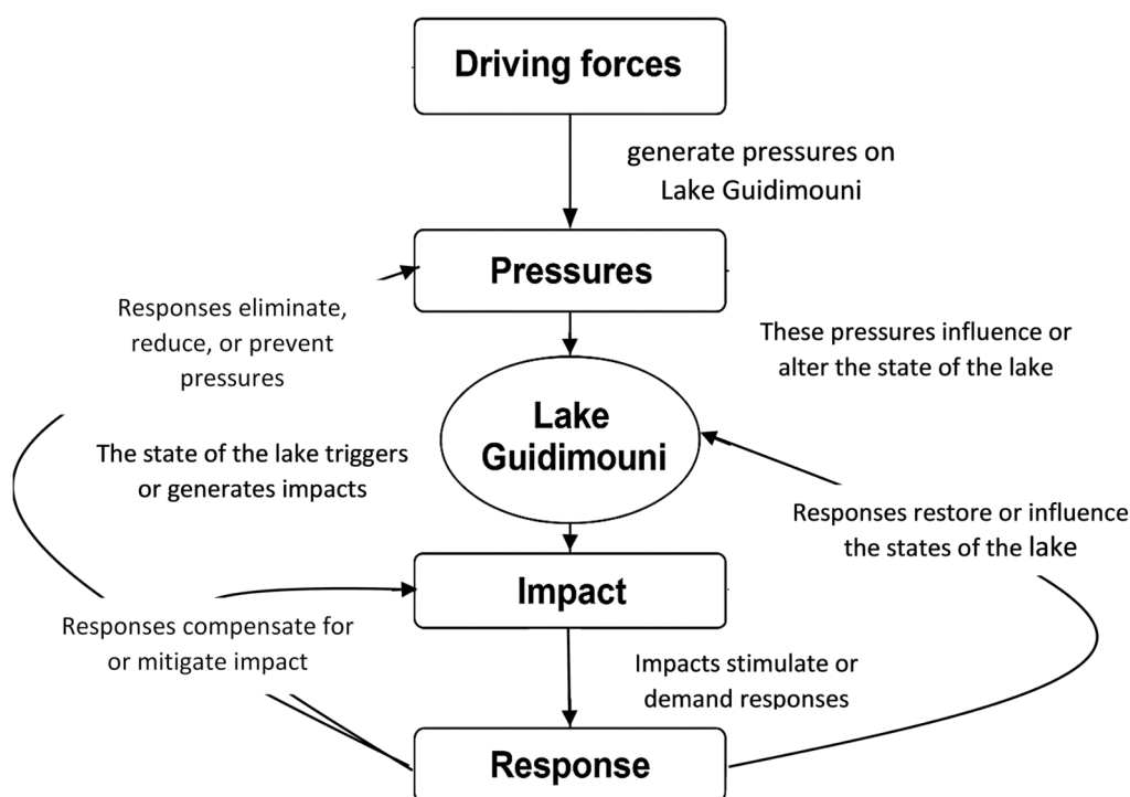
FIGURE 3 Operational DPSIR cycle linking climate drivers, ecological transitions and resilience responses in the Lake Guidimouni socio-ecological system. Schematic representation of the DPSIR (Drivers–Pressures–State–Impacts–Responses) cycle as explicitly operationalised for Lake Guidimouni to diagnose climate-driven socio-ecological change and identify leverage points for resilience. Drivers encompass both climatic and anthropogenic forcing factors, including increasing rainfall variability, intensifying flood–drought alternation, rising temperatures and land-use intensification. These drivers generate multiple Pressures, notably recurrent inundation, hydrological instability, sediment redistribution and the invasive expansion of Typha domingensis . The cumulative effects of these pressures reshape the ecological State of the lake, characterised by the transition from open-water and irrigated agricultural systems toward Typha -dominated marshlands, reduced habitat heterogeneity and declining land accessibility. These altered states translate into cascading Impacts on ecosystem functioning and human wellbeing, including loss of irrigable land, reduced agricultural productivity, biodiversity degradation, increased labour constraints, livelihood insecurity and heightened exposure to climate-related risks. Responses represent adaptive and mitigation strategies identified through the combined analysis of spatial evidence and convergent stakeholder perceptions. These include selective mechanical removal of Typha domingensis , hydrological regulation, adaptive land-use planning, livelihood diversification and participatory governance mechanisms aimed at restoring ecological balance and strengthening socio-ecological resilience. Bidirectional arrows highlight feedback loops and non-linear interactions within the DPSIR cycle, emphasising that responses may modify future pressures and drivers, thereby reinforcing or alleviating vulnerability. The figure synthesises the conceptual backbone of the DPSIR–GIS framework used in this study and underpins the spatial analyses, vulnerability mapping and resilience pathways developed for Lake Guidimouni between 2013 and 2024.
