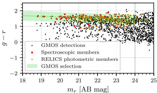
Figure 4. Colour-magnitude diagram of Gemini-N /GMOS sources (black dots). The red sequence is clearly visible in the g - r colour which straddles the 4000 Å-break at the cluster redshift z_d = 0.432 . We show the GMOS colours of known spectroscopic cluster members in red and of HST photometry-based cluster members in orange. Our GMOS red sequence selection window is shown in green.
