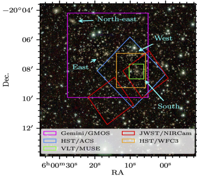
Figure 2. Cut-out of a VIRCAM colour-composite image (blue: Y band, green: J band, red: Ks band) overlaid with the field of views of the various observations of the MACS0600 used in this work (see Sections 2.1, 2.2, 2.3, 2.4, and 2.6).
