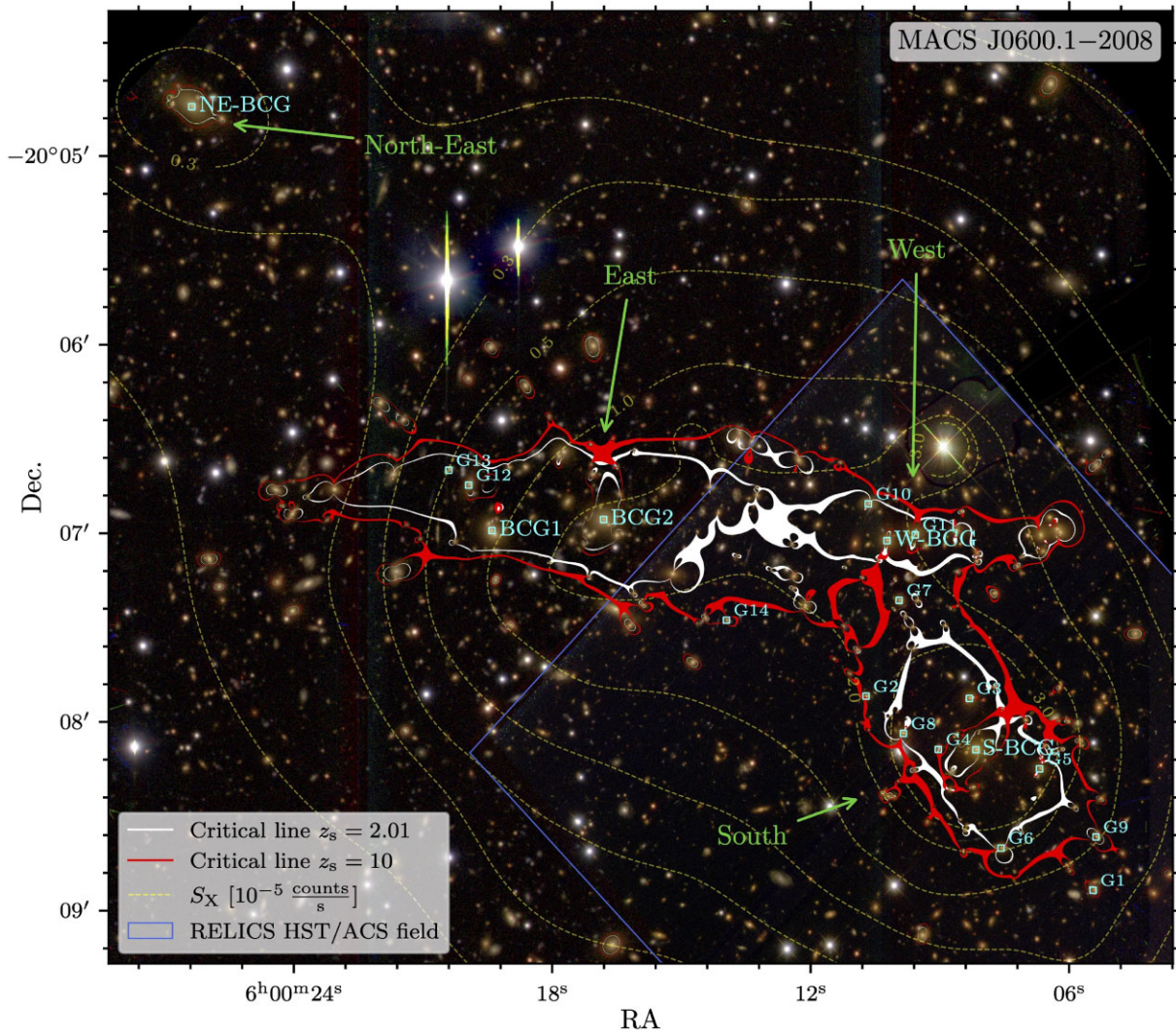
Figure 1. Combined HST /ACS and Gemini-N/GMOS composite-colour image (blue: g + F435W , green: r + F606W , red: i + F814W ) of MACS0600. The BCGs of the cluster (Section 3.1) and a number of cluster member galaxies of interest (see Table 2) are shown in cyan. Overlaid are the critical curves of our SL model (Section 4.3) for z_s = 2.01 (corresponding to system 1) and z_s = 10 in white and red, respectively. The green arrows designate the various cluster substructures analysed in this work. The X-ray surface brightness (see Sections 2.6 and 4.2, and Fig. 6) is overlaid as yellow contours in steps of [0.1, 0.2, 0.3, 0.5, 1.0, 2.0, 3.0] \times 10^{-5} \text{ counts s}^{-1} . The RELICS HST /ACS field of view (Section 2.3) is shown in blue. We nickname MACS0600 ‘Anglerfish cluster’ analogous to the deep-sea creature of which often only one part is immediately seen and the bulk remains hidden. A full-resolution ( 0.06 \text{ arcsec pix}^{-1} ), fully vectorized version of this figure is included in the online supplementary material of this paper.
