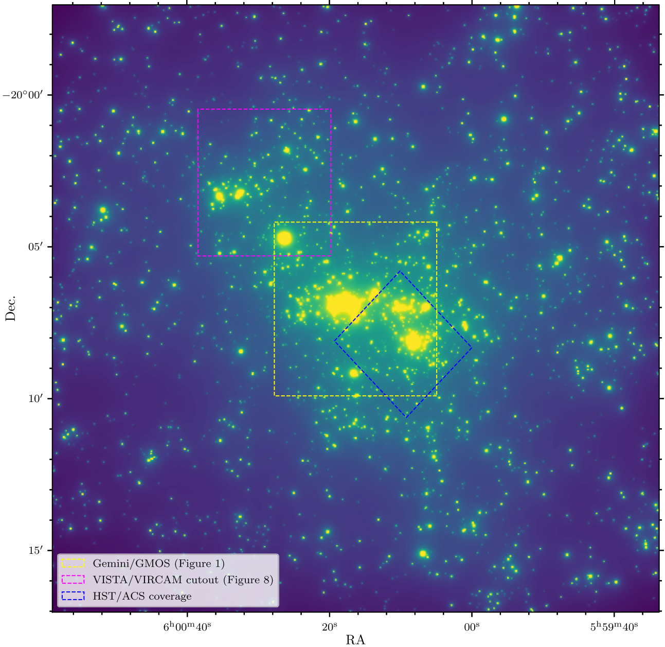
Figure 10. VIRCAM Y-band luminosity density of cluster member galaxies in a wide 20 arcmin \times 20 arcmin area around MACS0600. At z_d = 0.43 , one arcminute corresponds to 0.34 Mpc. While some 60 galaxies were verified spectroscopically (see Section 3.1), most of the cluster members were selected photometrically, some only in the VIRCAM imaging data with poor colour range, and should thus be referred to as mere candidates. The yellow square represents the area shown in Fig. 1, the magenta square the area shown in Fig. 9, and the blue square the previously known part of the cluster with RELICS HST coverage. The cluster member luminosity distribution presents an overdensity at roughly the same location as the northern X-ray structures shown in Figs 6 and 9, indicating that it indeed most likely lies at the same redshift and is associated with the cluster. Elongations of the luminosity density in the north-east to south-west, and tentatively towards the north-west direction, indicate filamentary structures with the cluster embedded in a node of the cosmic web.
