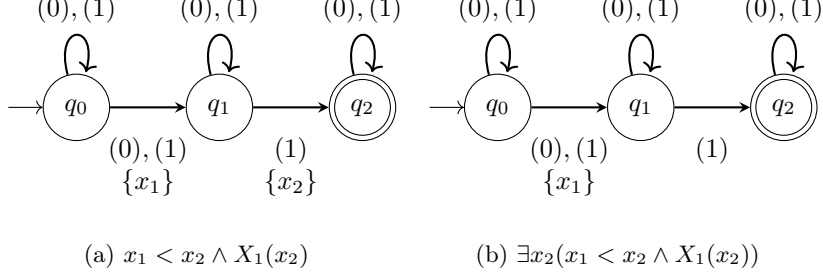
Figure 1: Automata recognizing sets of models.
