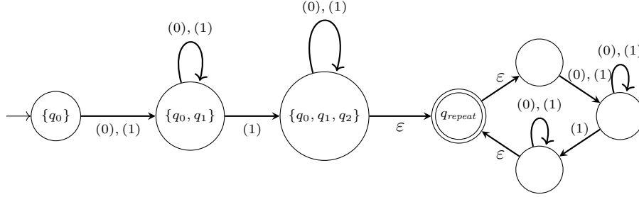
Figure 4: Automaton recognizing the set of models of \forall x_1 \exists x_2 (x_1 < x_2 \wedge X_1(x_2)) .
