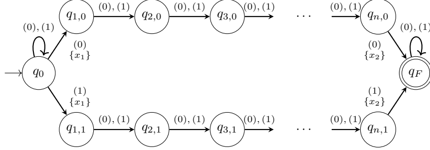
Figure 5: Automaton for x_2 = x_1 + n \wedge X_1(x_1) \Leftrightarrow X_1(x_2) .
