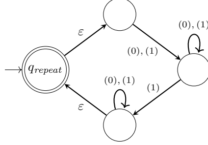
Figure 3: Widget for the state \{q_0, q_1, q_2\} .
