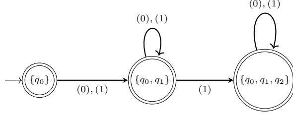
Figure 2: First step of construction for \forall x_1 \exists x_2 (x_1 < x_2 \wedge X_1(x_2)) .
