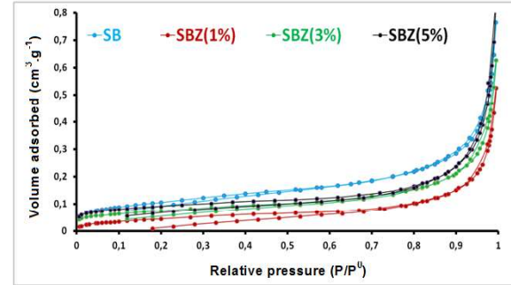
Figure 6. BET analysis of the fabricated photocatalysts.
