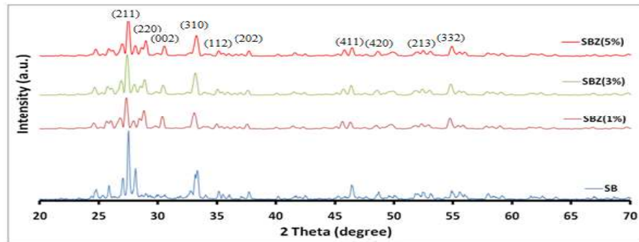
Figure 3. XRD patterns of pure and Zn-doped \text{SrBi}_2\text{O}_4 nanoparticles.
