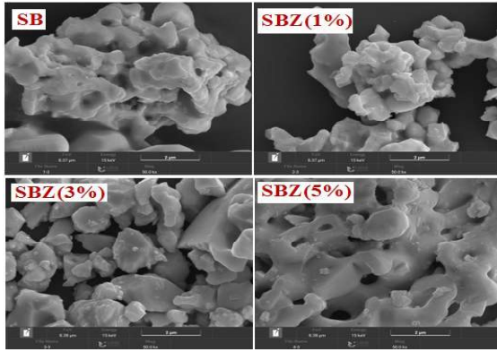
Figure 5. SEM micrographs of pure and doped \text{SrBi}_2\text{O}_4 .
