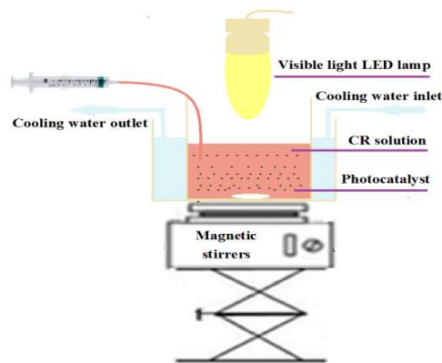
Figure 2. Schematic diagram of the photocatalytic device.
