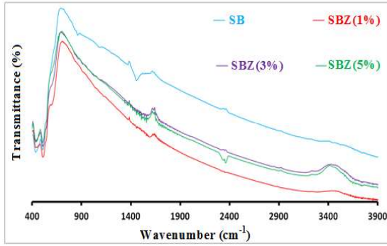
Figure 4. FTIR spectra of the photocatalysts.
