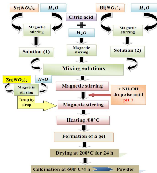
Figure 1. Diagram of the synthesis protocol of pure and Zn-doped \text{SrBi}_2\text{O}_4 by sol-gel process.
