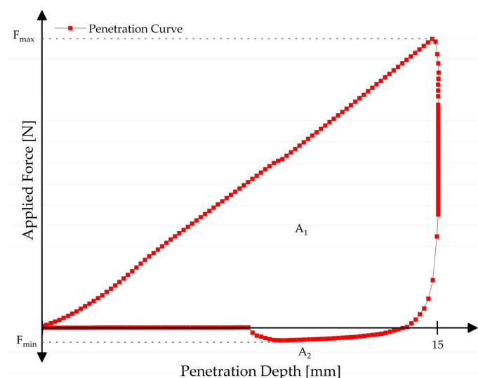
Figure 26. General results obtained from compression tests.
