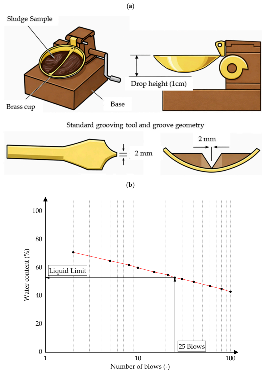
Figure 11. The Casagrande cup method: (a) Casagrande apparatus; (b) Casagrande classic results.
