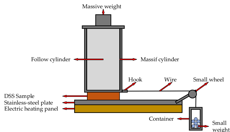
Figure 22. The Jenike test apparatus for DSS.
