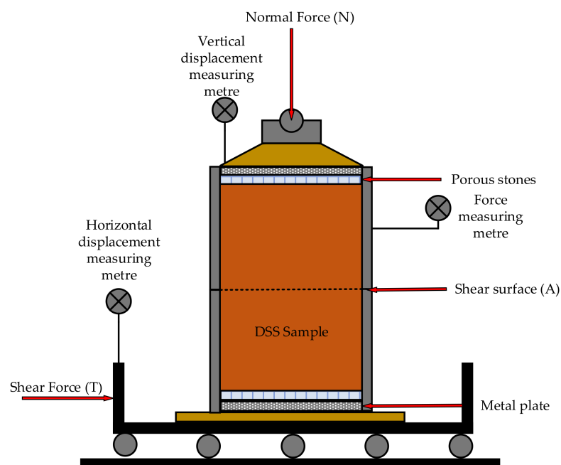
Figure 15. The direct box apparatus.
