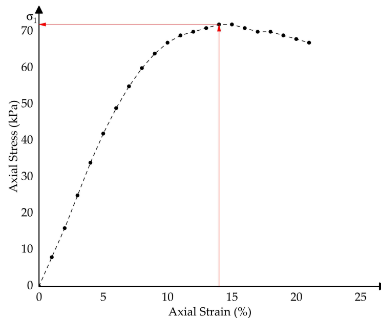
Figure 21. The unconfined test results.
