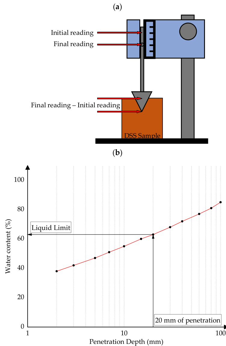
Figure 12. The cone penetrometer method: (a) cone penetrometer; (b) cone penetrometer classic results.
