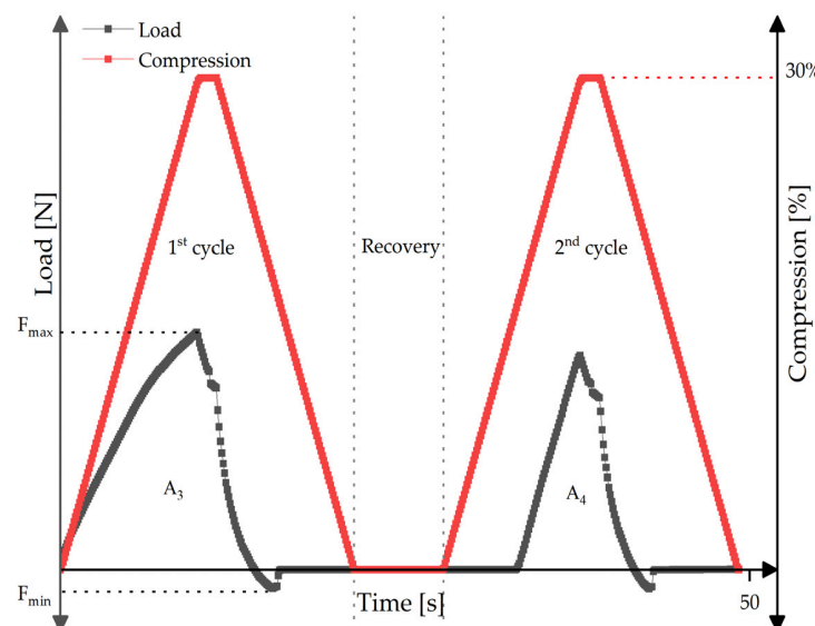
Figure 24. General results obtained from TPA tests.
