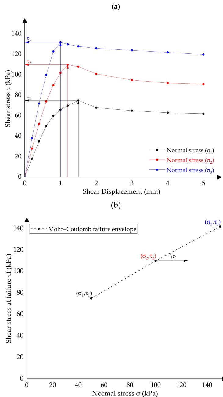
Figure 16. The direct box test results. (a) Shear stress–displacement curves under different normal stresses. (b) Mohr–Coulomb failure envelope: shear stress at failure vs. normal stress.
