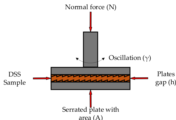
Figure 27. Oscillatory rheology tests schematics.
