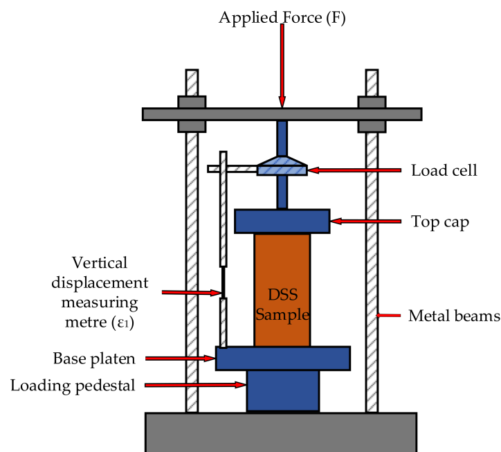
Figure 20. The unconfined compression test apparatus.
