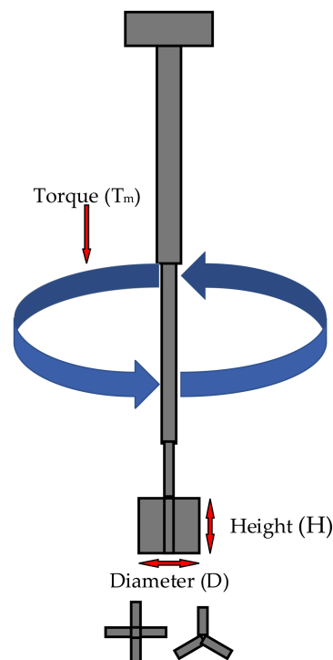
Figure 17. Vane shear test apparatus.
