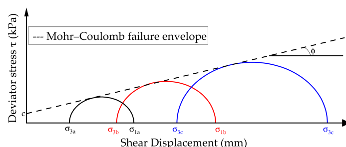
Figure 19. The triaxial test results.
