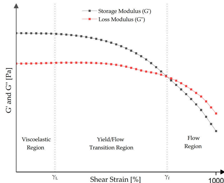
Figure 28. Oscillatory rheology tests general results.
