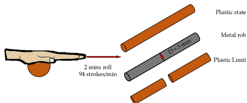
Figure 13. Plastic limit test.
