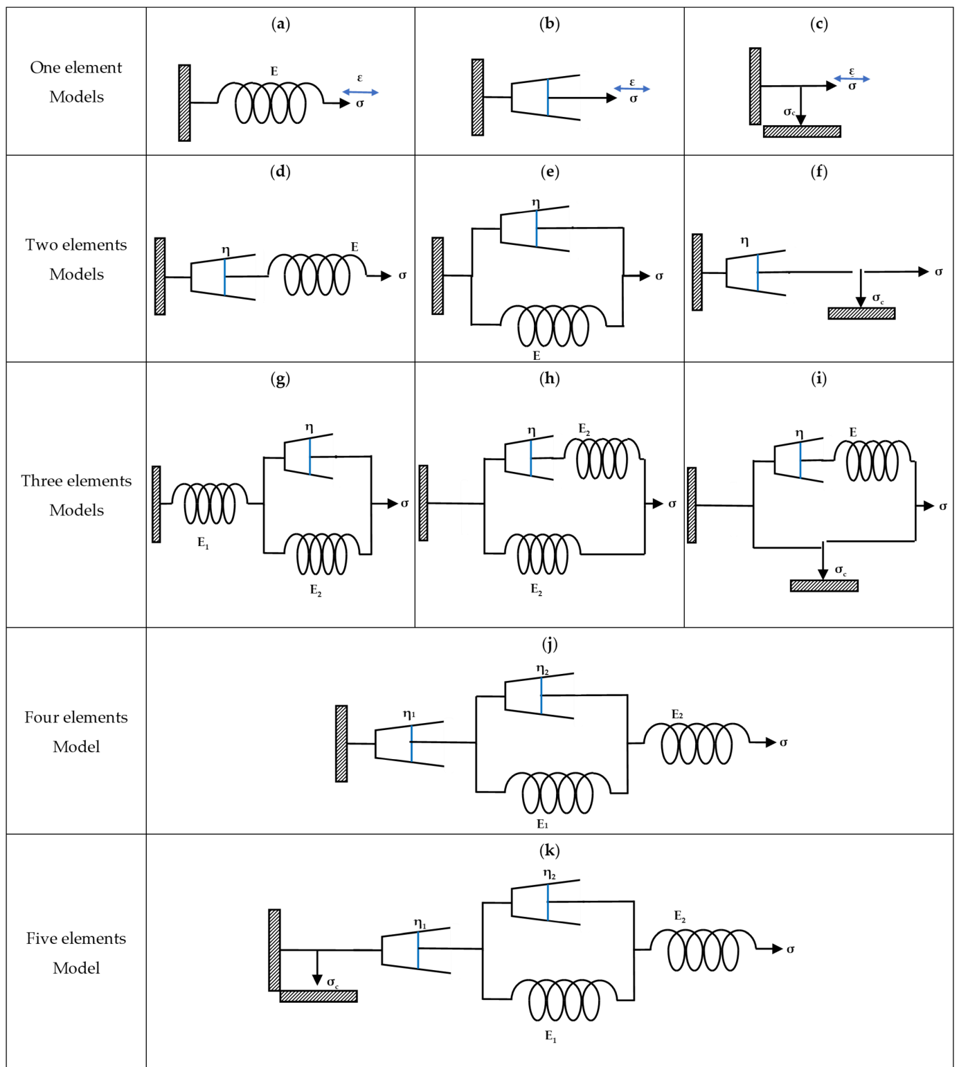
Figure 2. Hierarchical mechanical–analogue rheological models for characterizing DSS. (a) Hookean spring Model (Ideal elastic solid). (b) Newtonian dashpot Model (Ideal viscous liquid). (c) Friction slider Model (Ideal frictional solid). (d) Maxwell Model. (e) Kelvin-Voigt Model. (f) Bingham Model. (g) Terzaghi-Voigt Model. (h) Zener Model. (i) Bingham-elastic Model. (j) Burgers Model. (k) Burgers-Ludwik Model.
