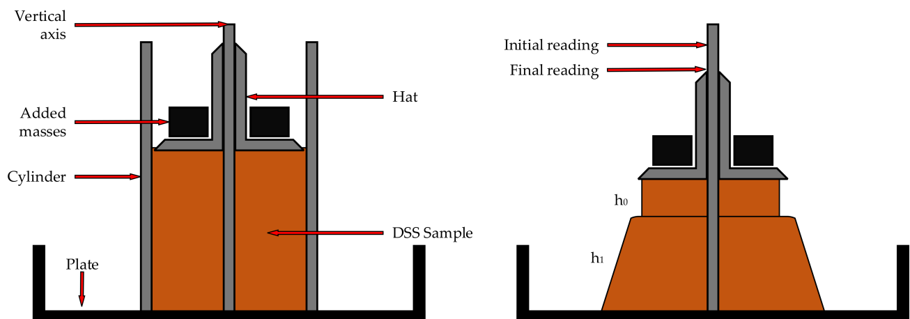
Figure 14. Baudez slump test evolution.
