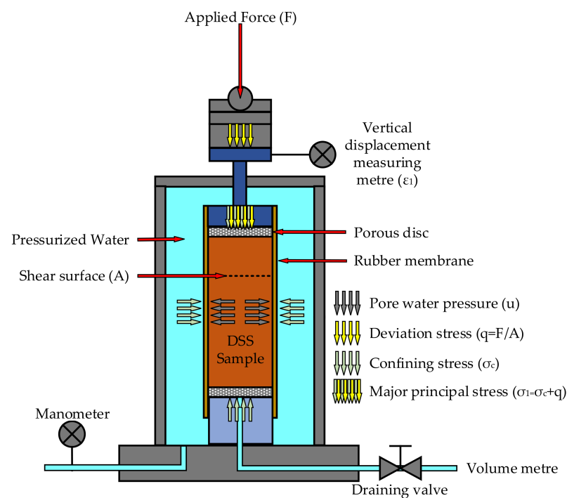
Figure 18. The triaxial apparatus.
