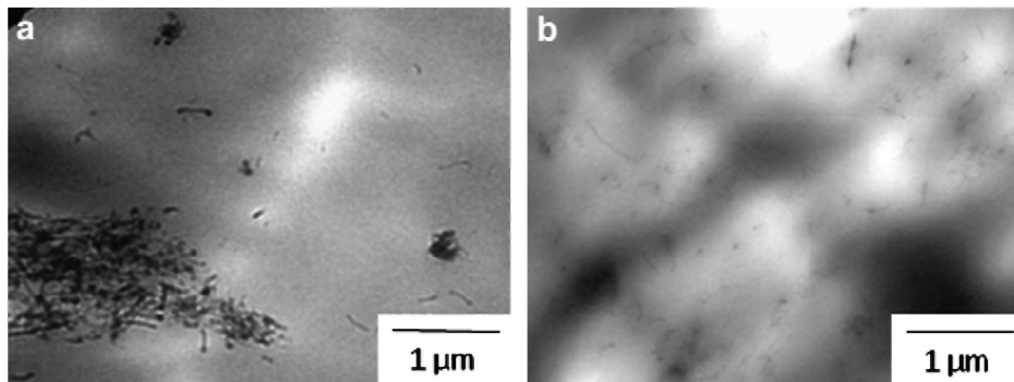
Fig. 7. TEM micrographs of (a) PP + 1% NT Thin and (b) PP + 10% PP-g-AMP + 1% NT thin (coprecipitation).
