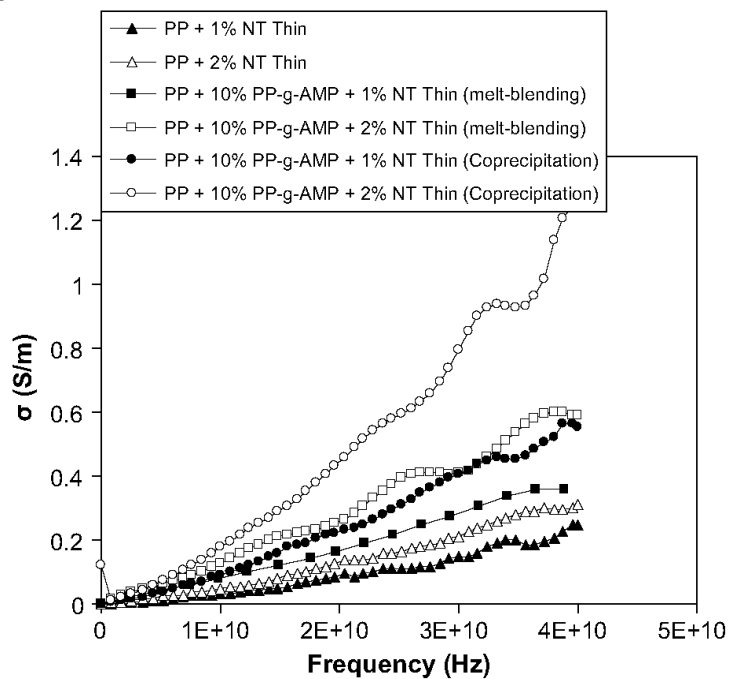
Fig. 11. Electrical conductivity as a function of frequency for PP/MWNT nanocomposites in the presence of PP-g-AMP.
