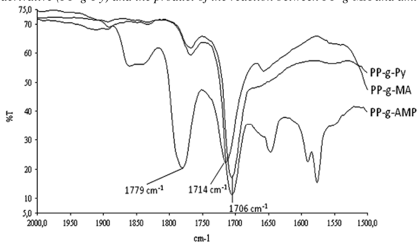
Fig. 2. FTIR spectra of PP-g-MA, the product of the reaction between PP-g-MA and the amino-pyrene derivative (PP-g-Py) and the product of the reaction between PP-g-MA and aminomethylpyridine (PP-g-AMP).
