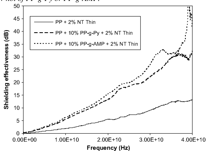
Fig. 12. Shielding Effectiveness (SE) as a function of frequency for PP/MWNT nanocomposites in the presence or not of PP-g-Py or PP-g-AMP.
