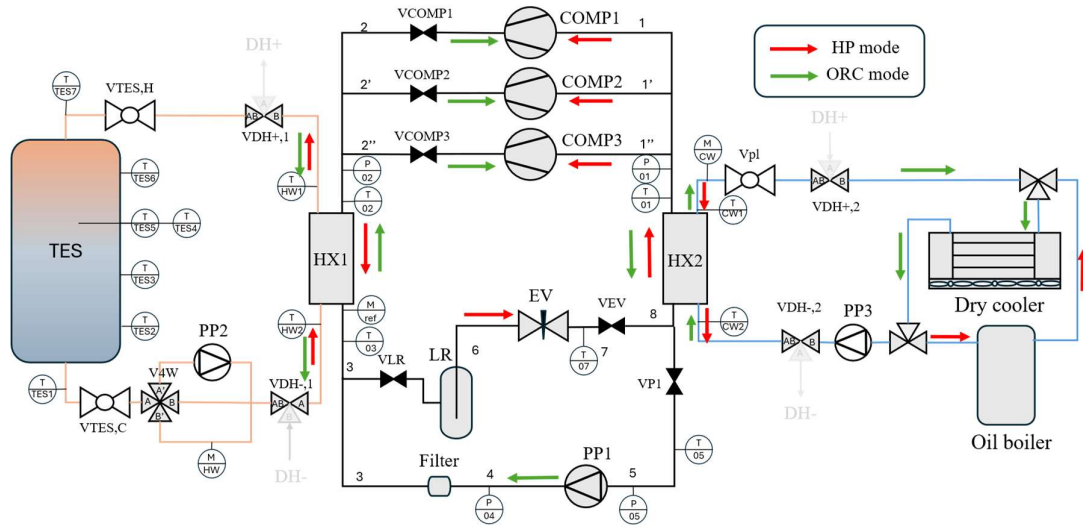
Figure 1. P&ID experimental set-up.
