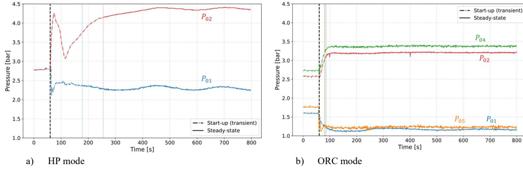
Figure 8. Comparison of pressure evolution in HP/ORC mode
