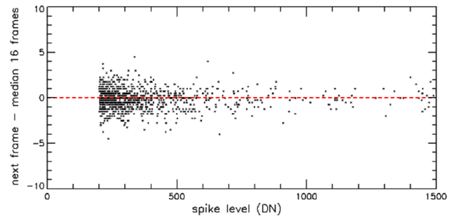
FIG. 14. Correlation plot between the level of a spike on a 18 \mu\text{m} pixel (up to 1500 DN, \sim 50\,000\text{ e}^- , close to the full well) and the difference between the level of the next acquisition and the median of 16 frames in a series (excluding the spiked acquisition) acquired with 1 MHz readout and an integration time of 100 ms.
