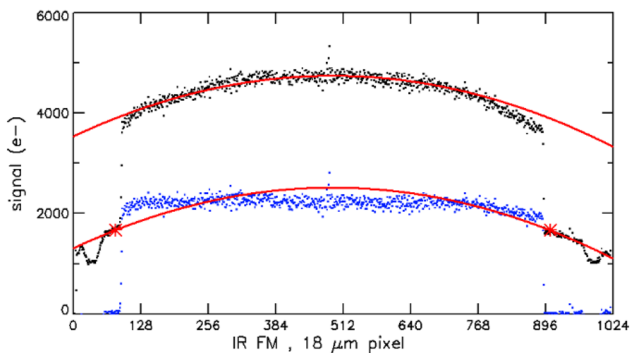
FIG. 26. Black dots: Spatial profile of spectel 5 (lowest wavelength not impacted by spillover; see Sec. II E). A parabolic fit (red curves) works well for both the signal in the FOV and the signal out of the FOV, with a near constant offset corresponding to the legitimate signal, expected to be flat. The legitimate signal (blue dots) has been evaluated by subtracting the spurious signal determined at the two reference locations close to the edge of the FOV (red stars) with a coefficient defined by the parabolic fit.
