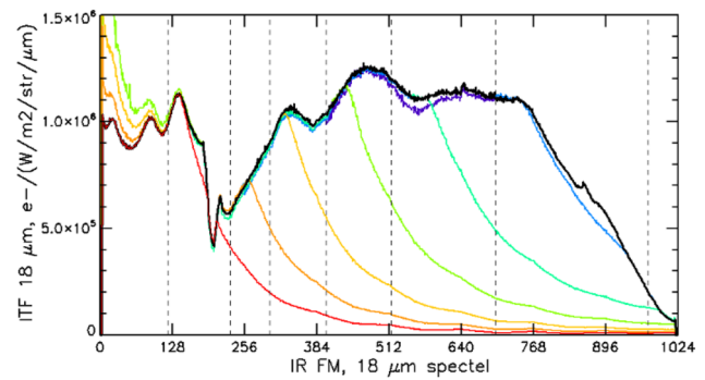
FIG. 20. Median ITF for pixels 500–520 (100 kHz readout, 800 ms, IR FPA at 88 K) obtained for each blackbody temperature by dividing the signal in \text{e}^- by the modeled radiance and the integration time. The results are consistent within a few percentage at domain boundaries. An interpolation with weights from 1 to 0 and 0 to 1 for the two relevant temperatures was applied across a range of 20 spectels so as to avoid small steps at domain boundaries when constructing the composite ITF (black line).
