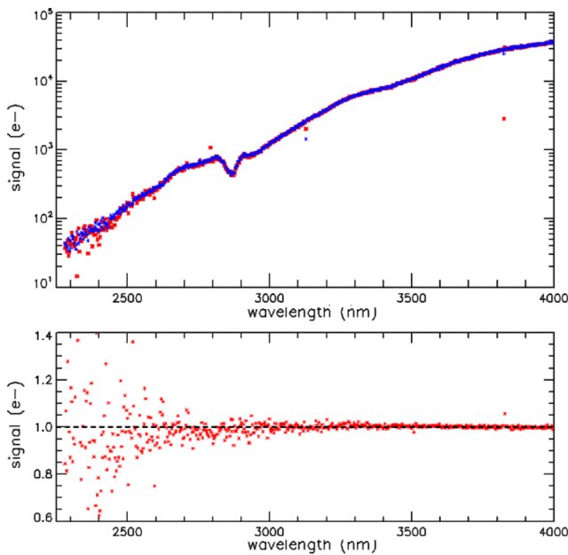
FIG. 29. Top panel: Dark-subtracted signal (16 frames average) for 18\text{ }\mu\text{m} pixel 512 of the IR FM detector with the blackbody at +10\text{ }^{\circ}\text{C} for an integration time of 100 ms (1 MHz readout) up to 4000 nm. The blue and red dots correspond to a temperature of the FPA of 88 K (blue) and 100 K (red). The stragglers correspond to unreliable hot spectels. Bottom panel: Ratio between the signal measured with the detector at 100 K and 88 K.
