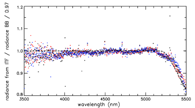
FIG. 30. Comparison of the Planck radiances ( \times 0.97 ) with the radiances determined for 18\text{ }\mu\text{m} pixels 150 (blue dots), 510 (black dots), and 850 (red dots) for a blackbody at -80\text{ }^{\circ}\text{C} with 1 MHz readout, an integration time of 100 ms, and the FPA at 100 K. The radiances have been evaluated using the 2D ITF for 1 MHz readout determined at 88 K. The black dashed curve corresponds to the results of a model 18 for the decrease in the quantum efficiency close to the cutoff wavelength of a detector.
