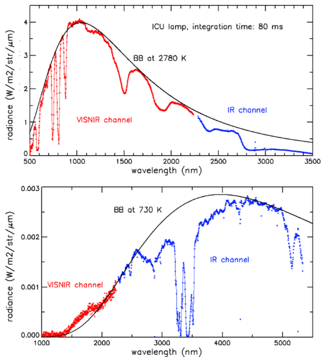
FIG. 41. Radiance profile obtained with both channels for the ICU lamp (top panel) and the ICU blackbody (bottom panel) after subtracting a modeled stray light contribution in the short wavelength range of the VISNIR channel. The observed radiance profiles indicate color temperatures in the range of 2780 K for the ICU lamp and 730 K for the ICU blackbody. The signal from the ICU blackbody is very low in the VISNIR channel.
